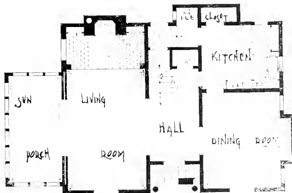
Plan of First Floor
