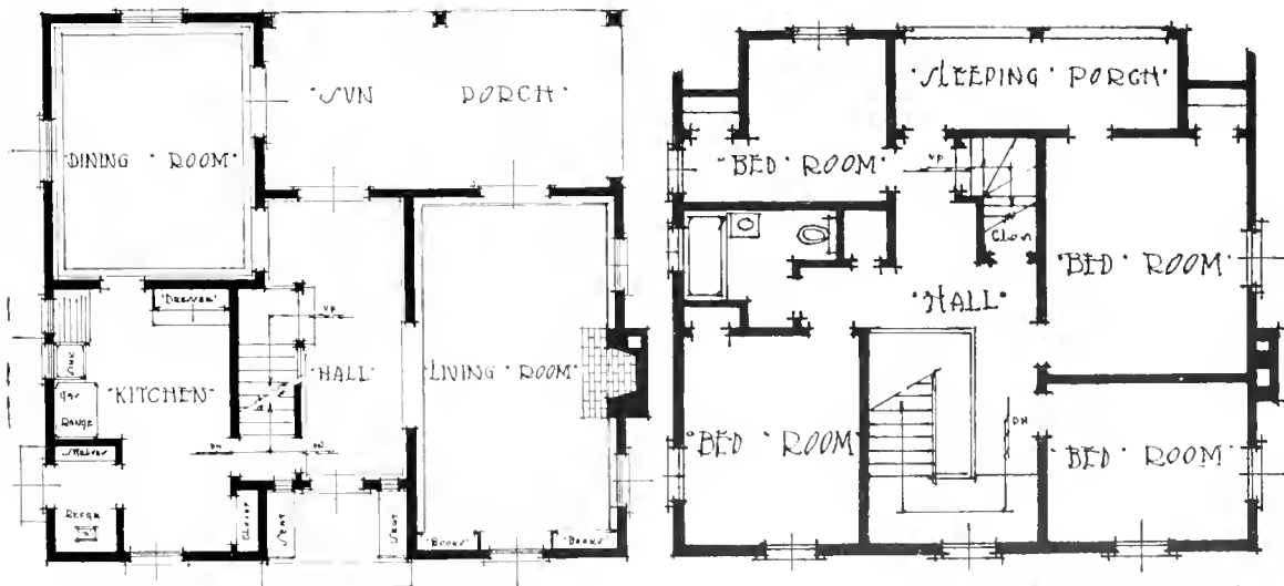
Plans of First and Second Floors
