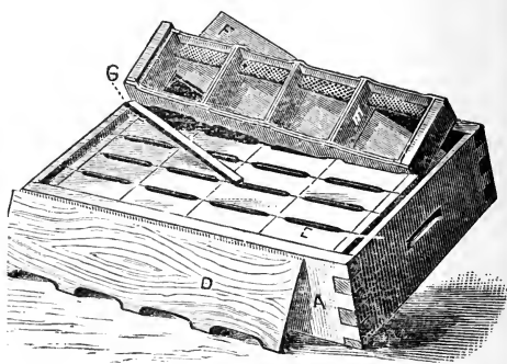
FIG. 57.—Super with sections and section holders in place: A, super; D, separator; F, sections; G, follower; G, wedge. (From Gleanings.)
