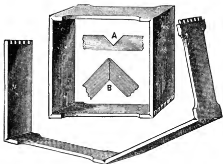
FIG. 56.—One-piece V-grooved sections. (From Gleanings.)
