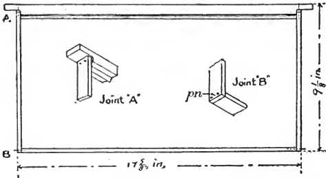
FIG. 24.—Langstroth frame; size, 17\frac{3}{8} in. by 9\frac{1}{8} in. outside; pn , projecting nail. (Original.)
