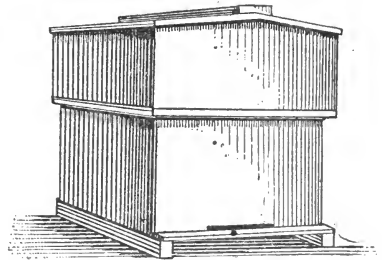
FIG. 74.—Double-walled hive adapted to outdoor wintering as well as summer use below 40° north latitude in the United States. Thickness of each wall, \frac{3}{8} inch; space between walls, 2 inches, packed with dry chaff or ground cork. (Original.)
