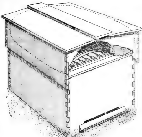
FIG. 26.—Lock-joint chaff hive. (From Cleanings in Bee-Culture .)
