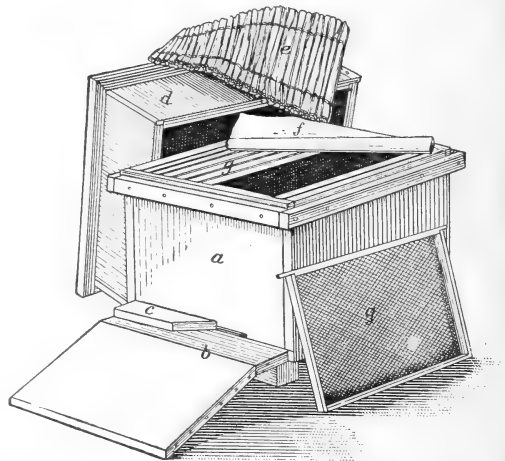
FIG. 31.—Dadant-Quinby form of Langstroth hive, open: a , front of brood apartment; b , alighting board; c , movable entrance block; d , cap; e , straw mat; f , carriage-cloth cover for frames; g, g , frames with combs. (From Langstroth.)
