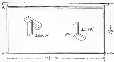
FIG. 24.—Langstroth frame; size, 17\frac{7}{8} in. by 9\frac{1}{8} in. outside; pn , projecting nail. (Original.)
