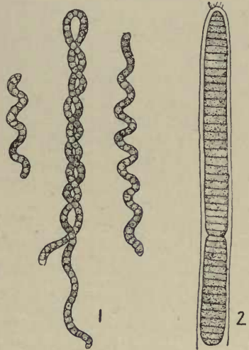
Fig. 480.—Blue-green Algae
