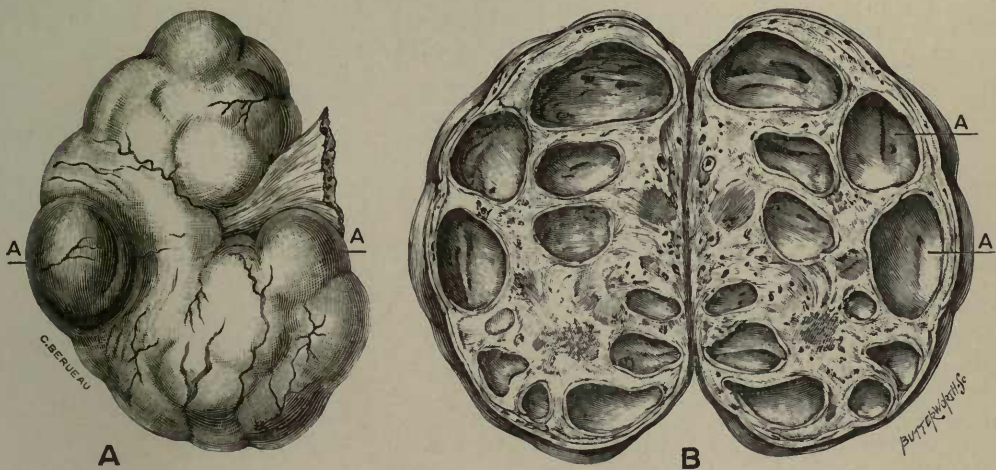
Fig. 527.—Cystic Ovary
