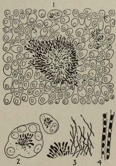
Fig. 477.—Actinomyces Bovis
