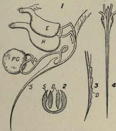
Fig. 459.—Wasp Sting
