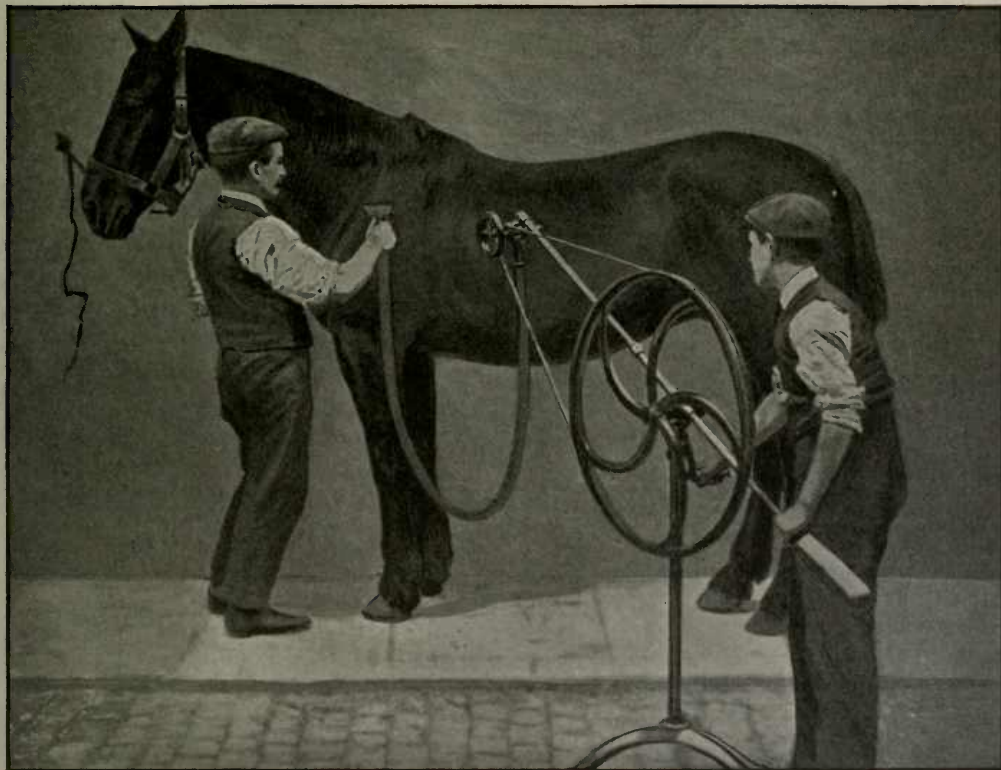
Fig. 487.—Barton-Gillette Clipping Machine
