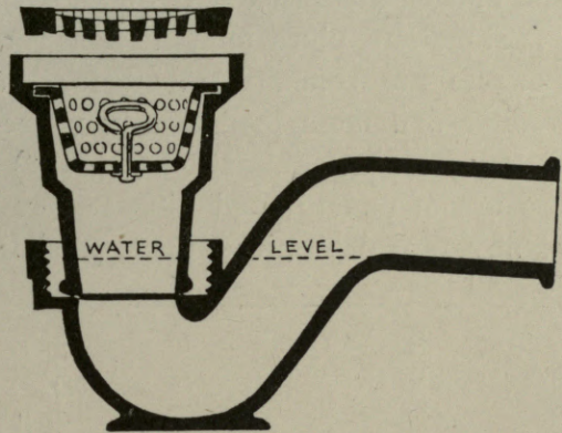
Fig. 474.—Winser's Iron Gully.
