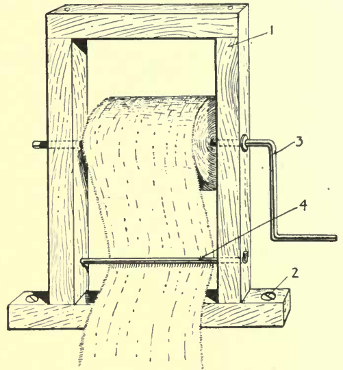
Fig. 449. A Simple Apparatus for Rolling Bandages 1, Wood framework. 2, Screw fixing to table or weight. 3, Bent stout wire crank. 4, Wire to guide and flatten bandage.
