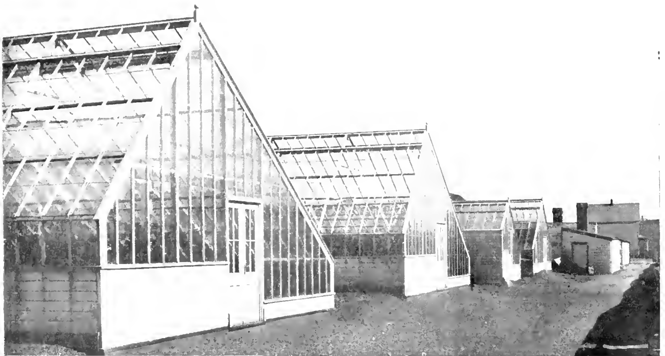
Gable view of the 30 foot Shadeless Ridge houses, with the old three-quarter span houses beyond.
