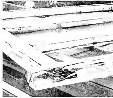
This is what happened to the side rail of an open mortise joint after the sash had been in use but nine years. Photo made the fifth of October, at Middle Village, L. I.
