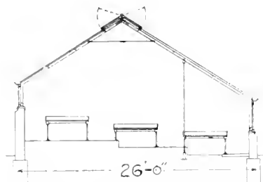
SECTION JOHN ASHE ROSE HOUSE
