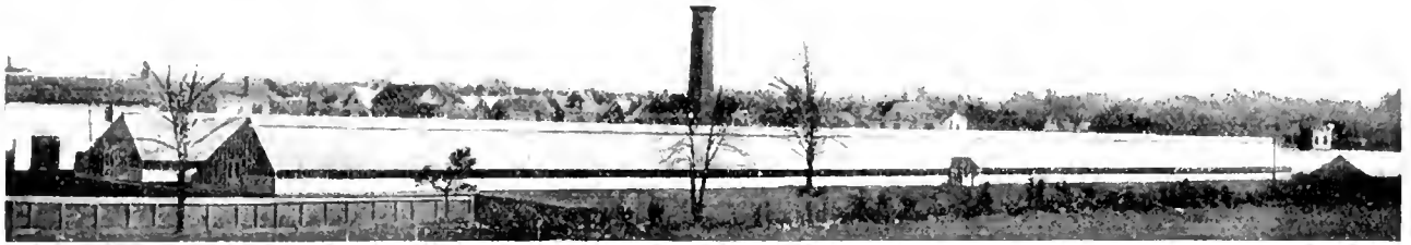
The two Sectional Iron Frame, Shadeless Ridge houses were erected in 1907. They are 465 feet long and 30 feet wide.
