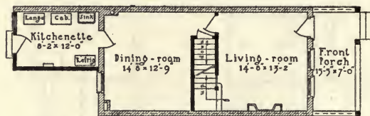
First-floor Plan
