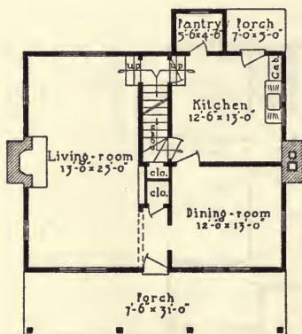
First-floor plan
