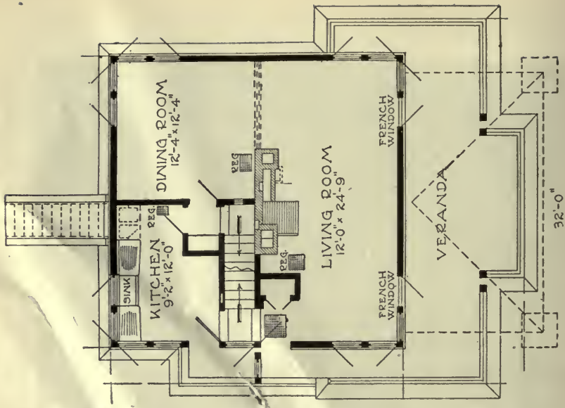
• FIRST STORY PLAN •
