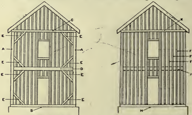
BRACED FRAME.
