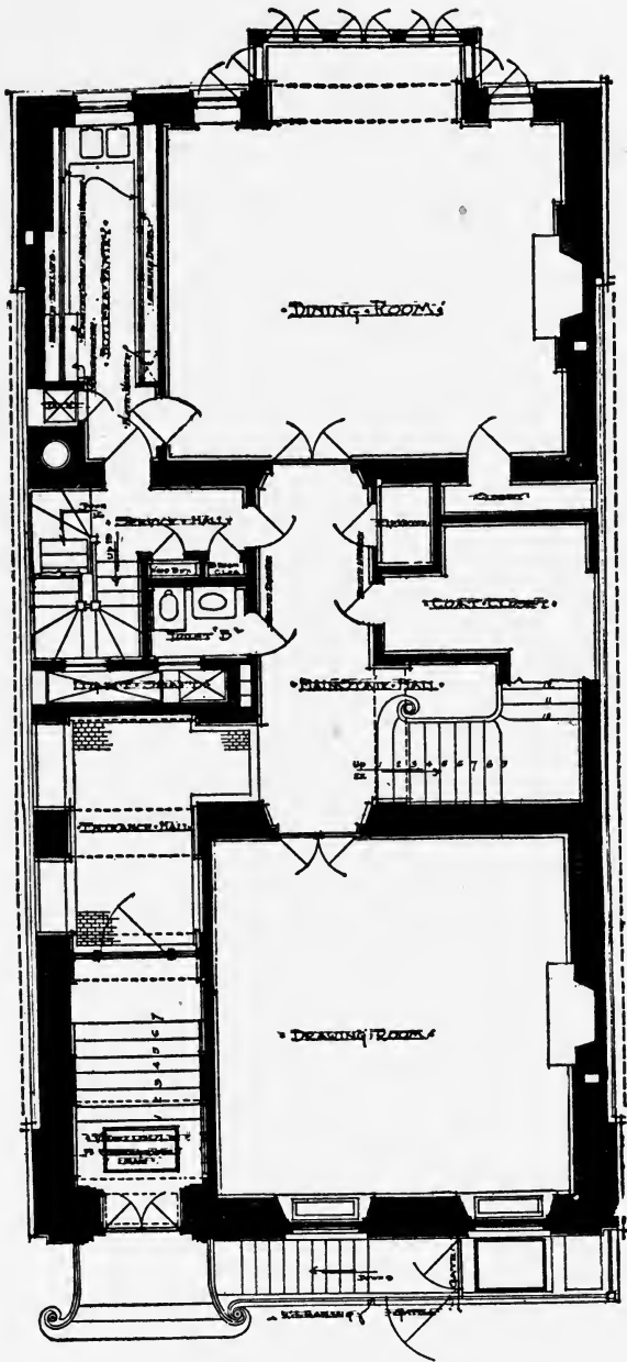
PLAN FOR A NARROW LOT
