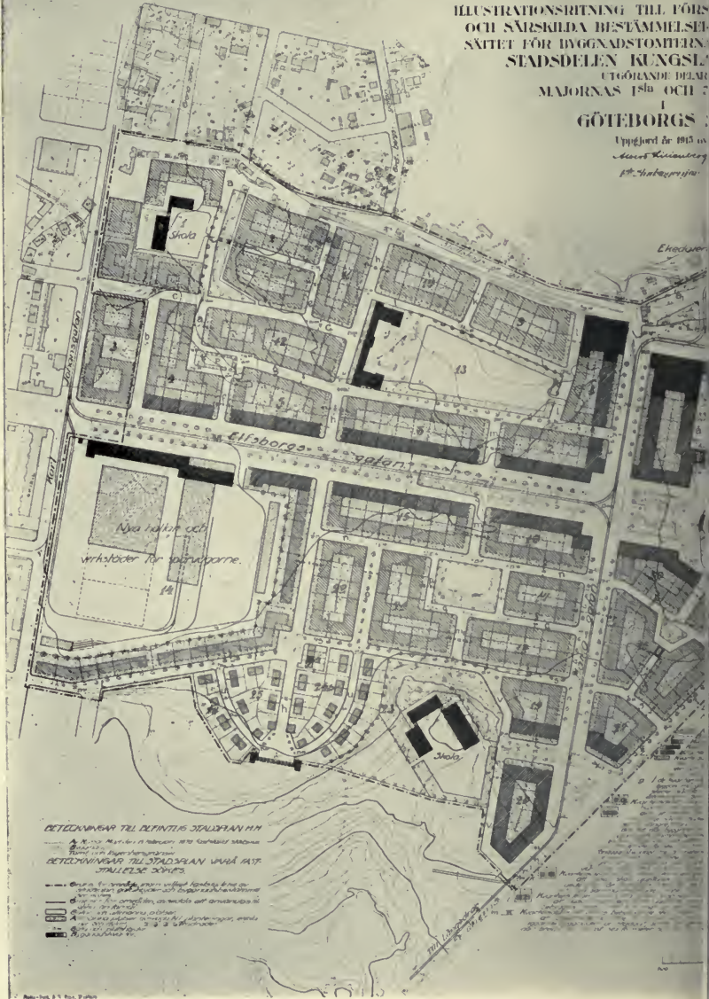
3. Part of the plan of Kungsladugård district at Gothenburg. The south-westerly rows; the western part to be the centre of buildings for public purposes and but there is an area
