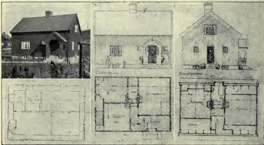
20. Municipal cottage, Gothenburg.
