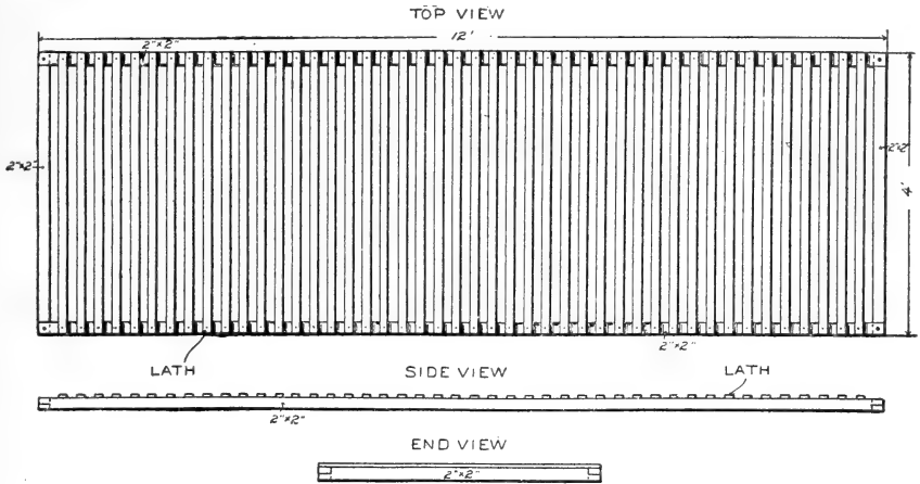
DIAGRAM 3.—Shade frame for seed bed, showing construction.
