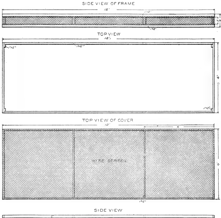
DIAGRAM 2.—Protective wire frame for seed bed, showing construction.
