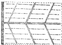
FIG. 76.—Plan for draining land.
