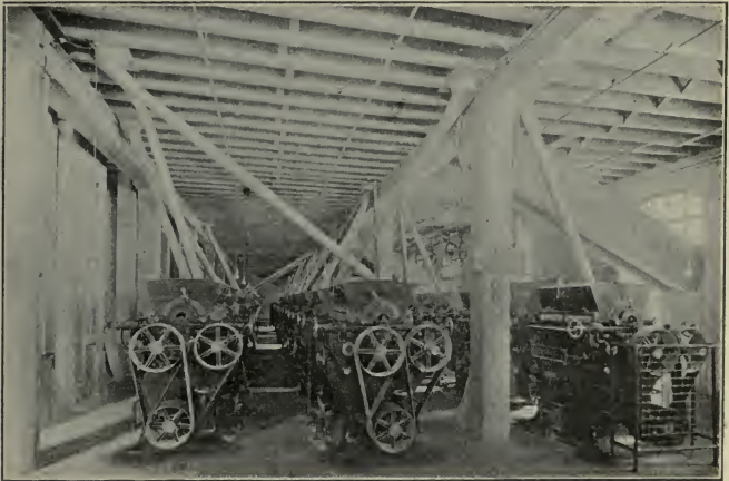
FIG. 7. — Grinding Wheat.
