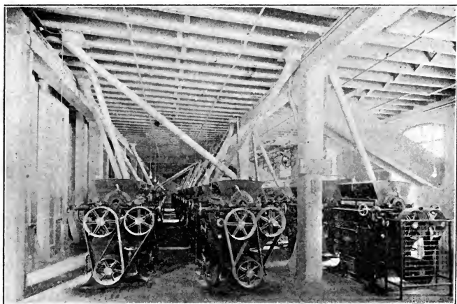
FIG. 7. — Grinding Wheat.
