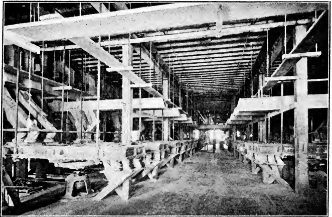
FIG. 8. — Bolting Flour.
