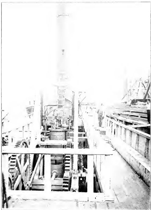
THE CLERMONT: INBOARD VIEW OF MACHINERY [567]
