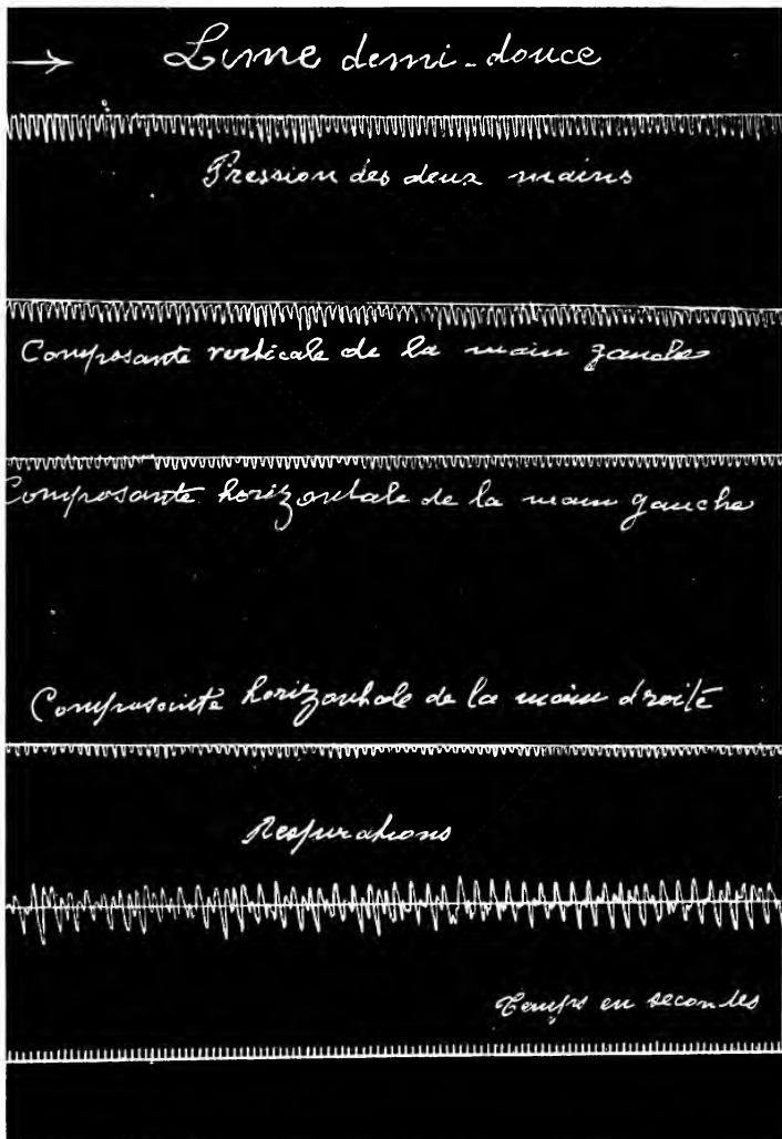
FIG. 13.—Records of physiological movements in the operation of filing by an experienced worker. From above downward the successive curves represent respectively: The vertical pressure of the two hands; the vertical pressure of the left hand; the horizontal pressure of the left hand; the horizontal pressure of the right hand; the respiratory movements; the time in seconds. (From Amar, Organisation Physiologique du Travail .)
