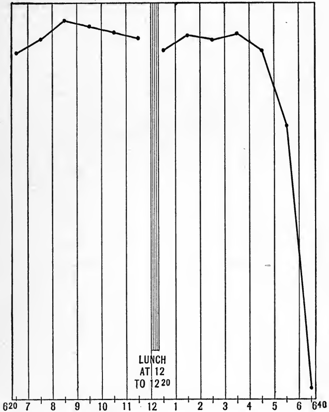
FIG. 6.—Curve of output in night work. The height of each point in the curve above the base line represents the output of the corresponding hour. Men workers; lathe operation; shift of twelve hours and twenty minutes. (By courtesy of the U. S. Public Health Service.)
