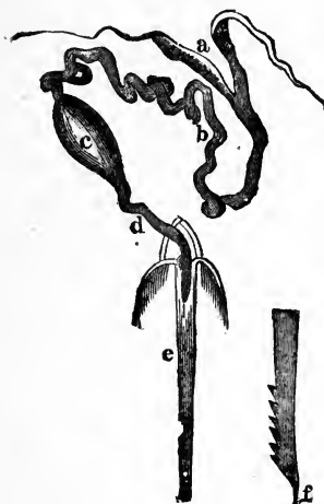
Fig. 5.—BEE STING.
