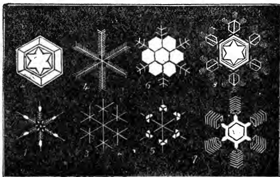
Fig. 1—SNOW CRYSTALS.
