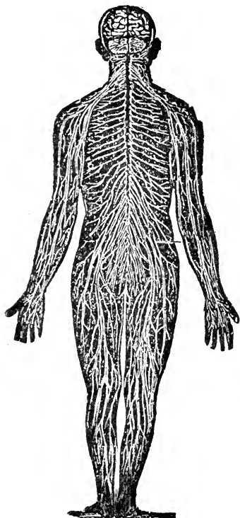
Fig. 16.—NERVOUS SYSTEM.
