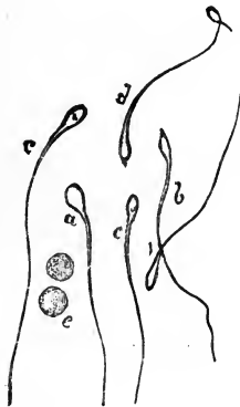
Fig. 62.—HUMAN SPERMATOZOA.*
