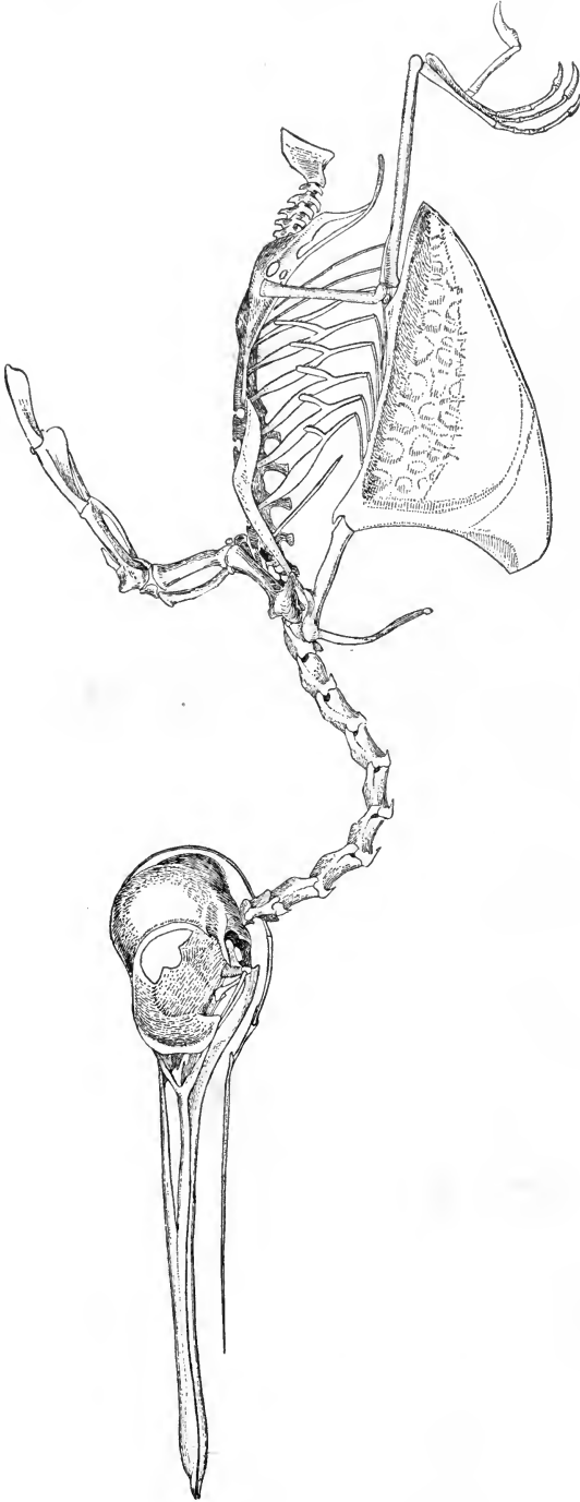
SKELETON of Trochilus colubris . (Enlarged 2½ times.)
