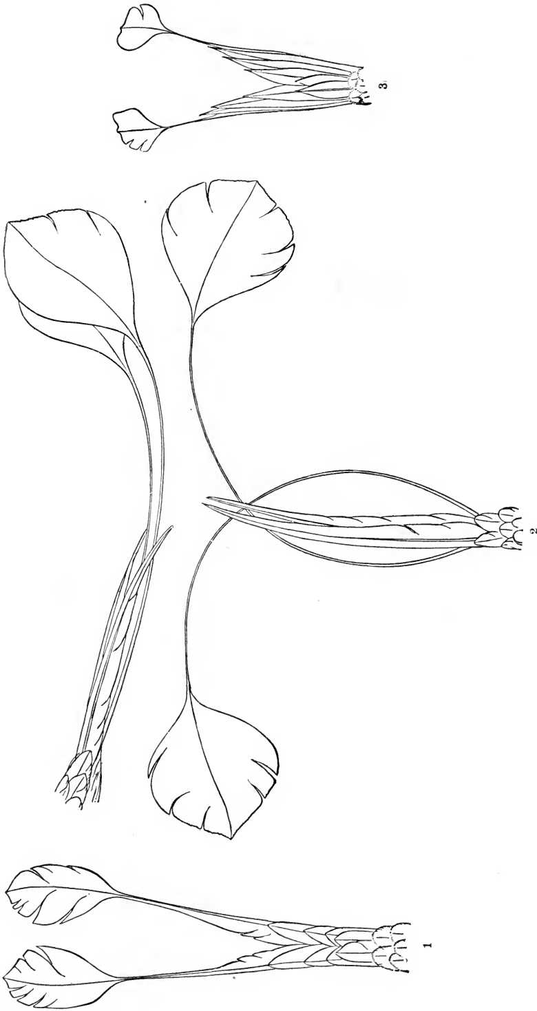
OUTLINES OF TAILS OF HUMMING BIRDS.
