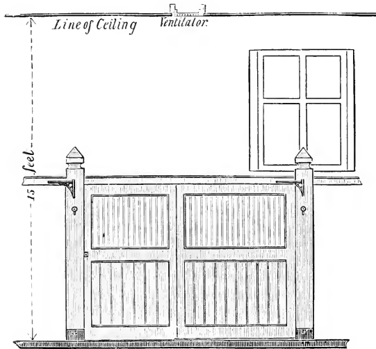
Elevation of Front of Loose Boxes, showing Height of Ceiling.
