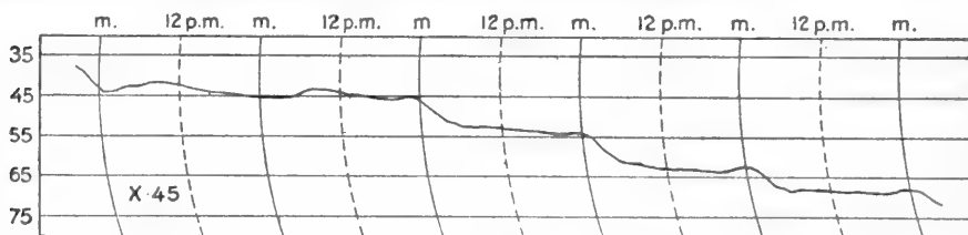
FIG. 25.—Tracing of auxographic record of variations in thickness of joint of Opuntia approaching maturity. Upward movement of pen denotes increase in thickness, \times 45 . Measurements made from place between areoles near base of joint. Scale ruled to 5 mm. and 12-hour intervals. It is to be noted that the hour is set forward on the summer schedule.
