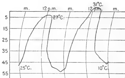
FIG. 37.—Variations in thickness of a mature leaf of Mesembryanthemum . X 45. Temperatures taken from a similar leaf with a mercurial thermometer.
