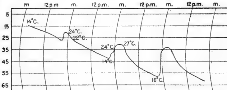
FIG. 35.—Auxographic record of thickness of pair of leaves about half mature size. X45. A daily shrinkage between 8 a. m. and midday occurred, which amounted to an increasing proportion of the increase taking place during the remainder of the day.
