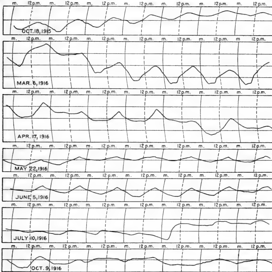
FIG. 28.—Portions of auxographic record of variations in length of a joint of Opuntia from October, 1915 to October of 1916. The joint had formed roots which depended in a glass jar of tap-water and the joint was held firmly in a natural erect position. The preparation stood in the south end of a glass house and was exposed to the alternations of sunlight and darkness with accompanying temperatures as low as 8° C. in the morning and as high as 45° C. in midsummer afternoons. The actual variations are amplified 30 and elongation is denoted by the downward movement of the pen. Divisions of scale = 1 cm. The joint was in a stage of completed growth during the week beginning October 18, 1915, at which time elongation occurred from evening until the middle of the forenoon, and shortening during the remainder of the day, with the length less at the end of the week than at the beginning. The records for March and April show a similar daily periodicity, but with an increase in length which may be ascribed to imbibition under the advancing temperatures. The daily losses and gains are more nearly equal in May and June and the variations of narrow amplitude. Some loss is shown in July and the reactions of the joint a year from the beginning of the record show a daily variation different in many particulars from those of the previous year. See figure 29 for a continuation of the record.
