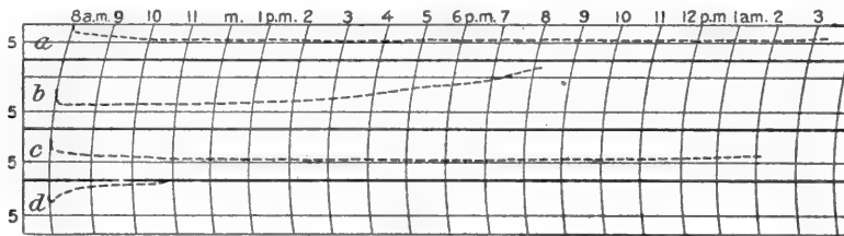
FIG. 18.—Swelling of tangential slices from tips of asparagus shoots at 14° to 17° C., X 20, on scale ruled to 5 mm. and 1-hour intervals. a, swelling of trio 3.8 mm. in thickness 7 per cent in water; b, swelling of trio 3.7 mm. in thickness 4 per cent in hundredth-normal citric acid; complete within a few minutes, followed by gradual shrinkage; c, swelling of trio of sections 6.2 per cent in sodium hydroxid with final shrinkage; d, slight swelling of trio of sections in hundredth-normal potassium chloride and hydrochloric acid and then rapid shrinkage.
