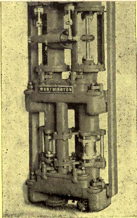
WORTHINGTON SINKING PUMP, WITH CHANNEL IRONS.
