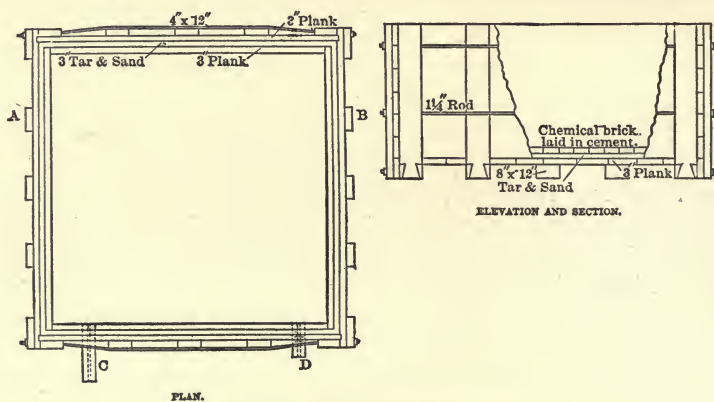
FIGS. 12 AND 13.—LIXIVIATION TANKS.
