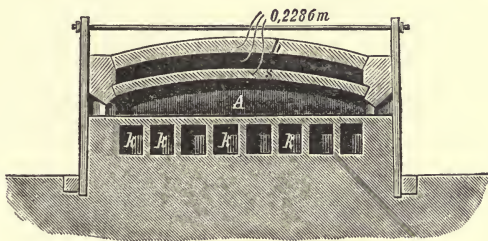
FIGS. 67 AND 68.—REVERBERATORY FURNACE OF THE BEDE METAL COMPANY.
