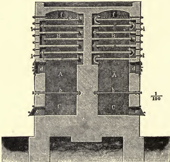
Vertical Section.
