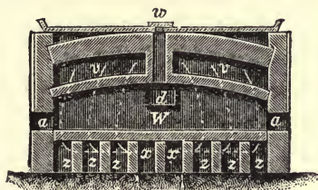
FIGS. 76 TO 78.—MUFFLE FURNACE USED BY THE THARSIS COMPANY.
