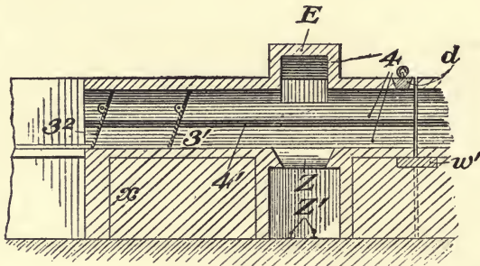
FIG. 105.—DISCHARGE OPENING OF THE BROWN ROASTING FURNACE.
