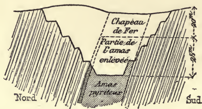
FIG. 6.—TRANSVERSE SECTION OF THE OPEN-CAST WORKINGS OF THE LAGUNAZO DEPOSIT.
