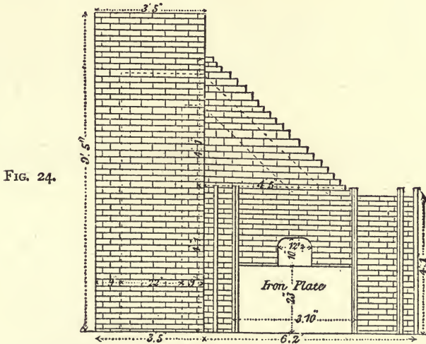
SECTIONAL VIEWS OF THE BOSTON AND COLORADO REFINING FURNACE.
