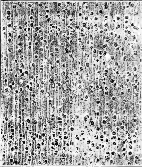
FIG. 5.—"AFRICAN MAHOGANY." END GRAIN MAGNIFIED 7.5 DIAMETERS.
