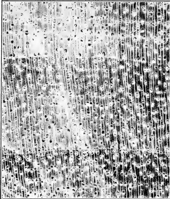
FIG. 11.—“WHITE MAHOGANY.” END GRAIN MAGNIFIED 7.5 DIAMETERS.
