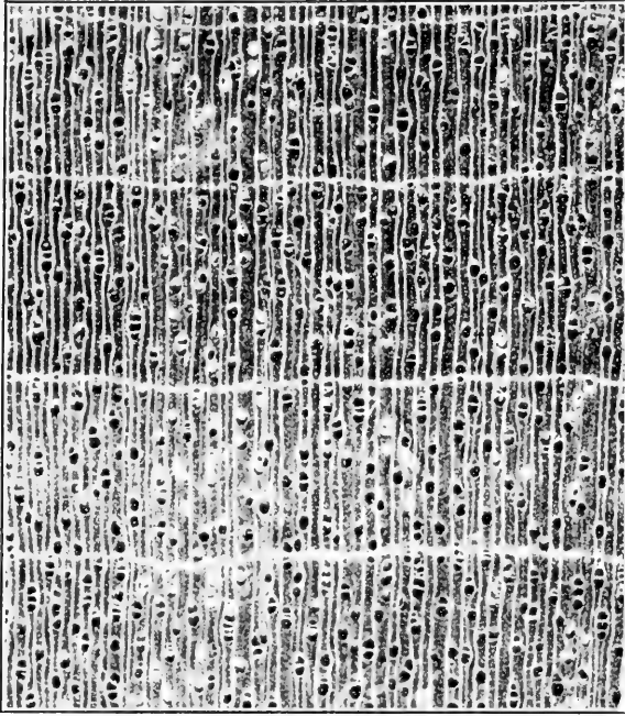
FIG. 1.—TRUE MAHOGANY. END GRAIN MAGNIFIED 7.5 DIAMETERS.
