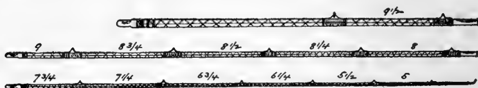
Guide and winding layout for 10-foot fly-rod
