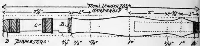
Fig. 4 — Wood grasp
