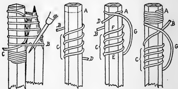
Fig. 6 Fig. 7 Fig. 8 Fig. 9 Silk winding: (6) Marlin-pin method; (7,8, and 9) Method in which terminal coils are thrown first around joint
