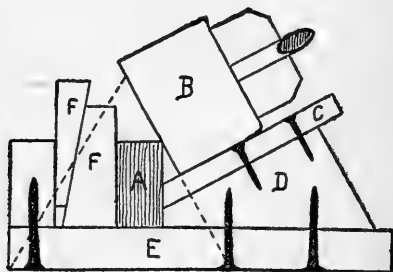
Pattern for planing-rig:
