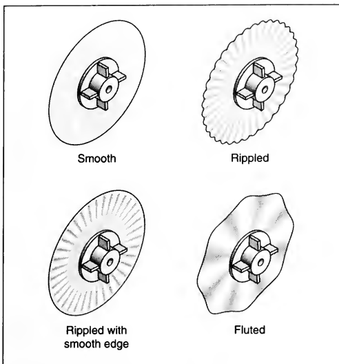
Figure 13.01. Common coulters styles.
