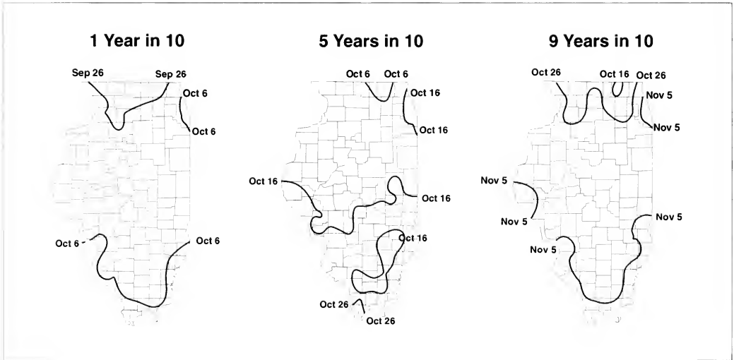
Figure 1.02. Probable dates of first fall frost (32°F minimum temperature).
