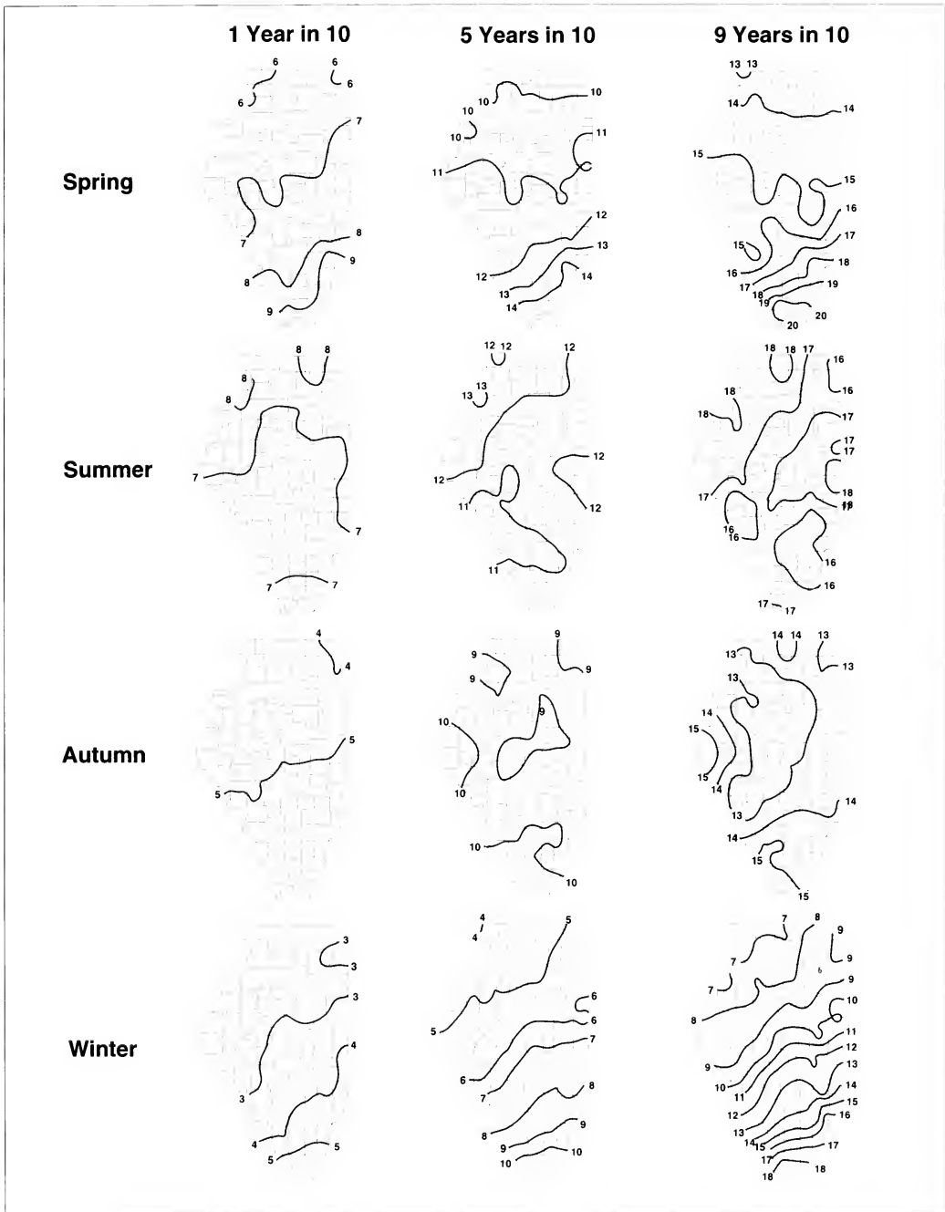
Figure 1.06. Probable seasonal rainfall amounts (inches).
