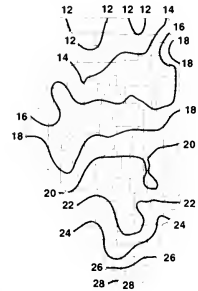
Figure 1.03. Mean maximum and minimum temperature for spring, summer, autumn, and winter.
