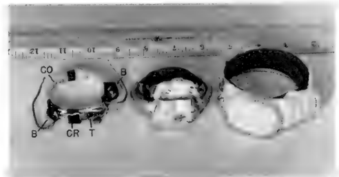
Three miniature tracking radio transmitters. The one on the left shows the principal parts (b, batteries; co, collar with antenna; cr, crystal; t, transistors). The middle transmitter has the parts partially imbedded, the one on the right has them completely imbedded and ready for use. These also represent three types used on different sized animals.
