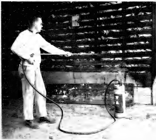
Hand equipment shown here is effective for applying insecticide sprays to corn in the crib.
