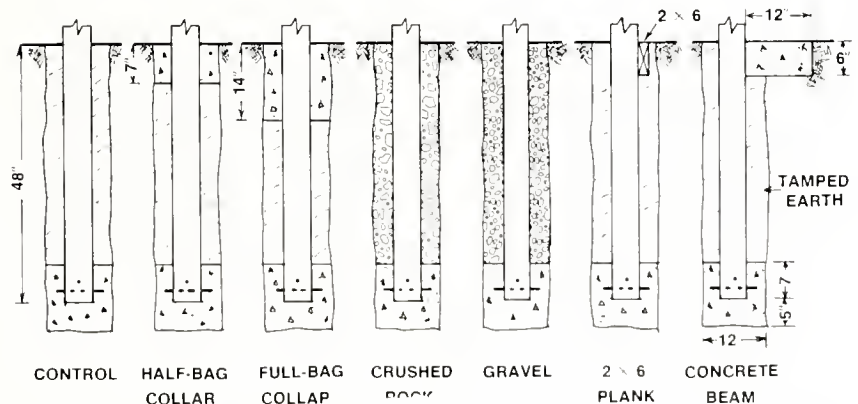
Types of post anchorage systems tested.
