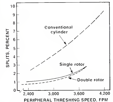
Effect of peripheral threshing speed on percentage of splits in clean-grain auger samples. Results were averaged from three harvest moisture levels of 13.3, 12.5, and 11.6 percent. (Fig. 1)
