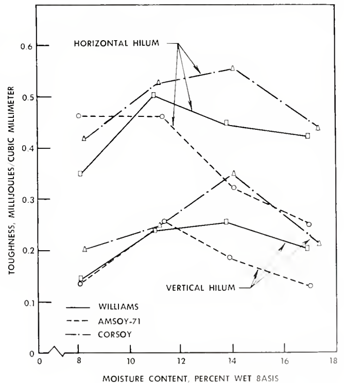
Toughness (energy per unit of volume) at seedcoat rupture as a function of moisture content for soybeans deformed at 1 millimeter per minute. (Fig. 4)
