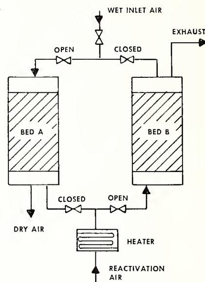
Typical dual-bed dehumidifier. (Fig. 1)
