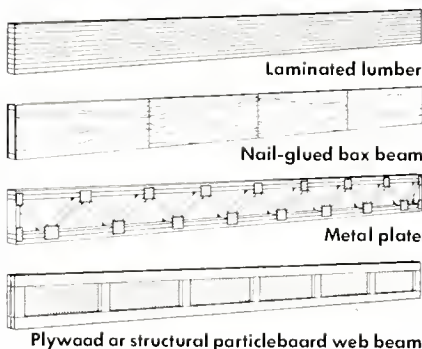
Four types of garage-door beams. (Fig. 2)
