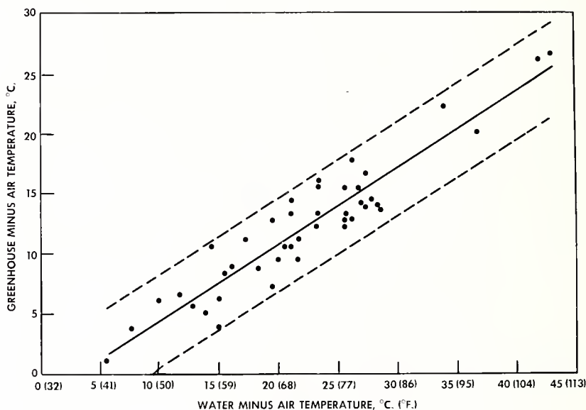
Greenhouse minus air temperature differential as a function of water minus air temperature differential. Dashed lines represent 95-percent confidence interval for actual values of ordinate. (Fig. 1)
