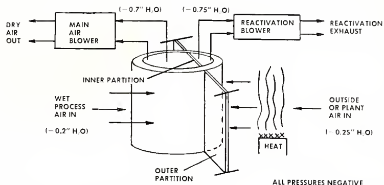
Rotating vertical drum-type dehumidifier. The desiccant is alternately cycled through two air streams.
