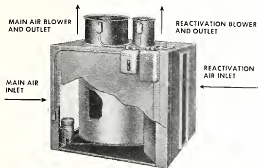
Rotating vertical drum-type dehumidifier. The desiccant is alternately cycled through two air streams.
