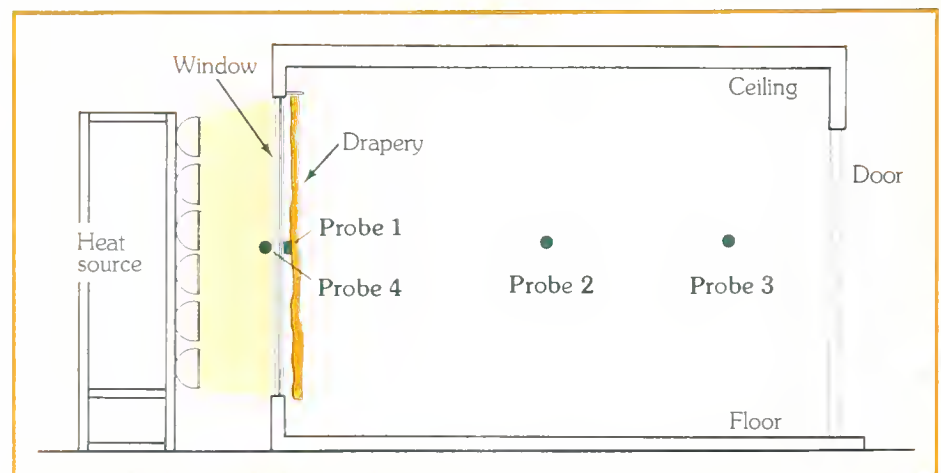
A diagram of the test room shows the location of four probes, which are attached to devices for monitoring variations in temperature and humidity. When charted, the variations indicate the insulation value of drapery fabrics and configurations.
