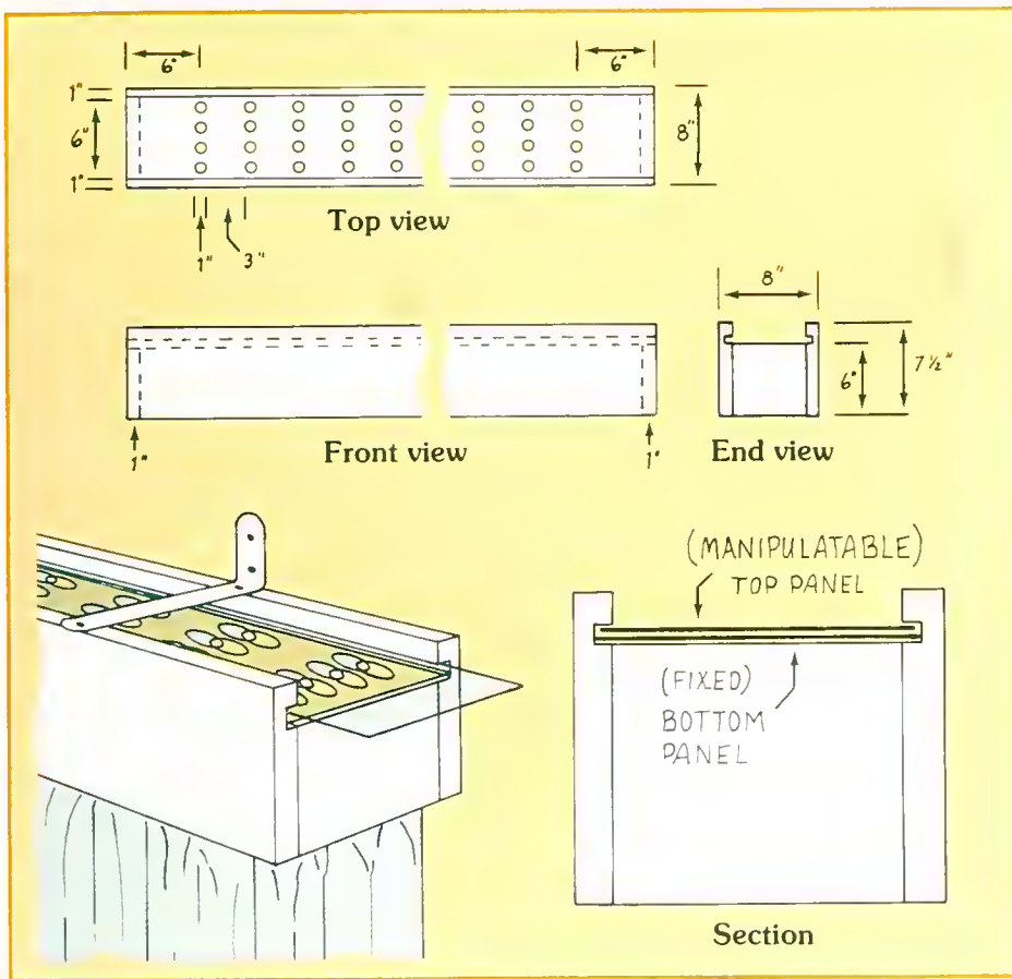
This sketch of the manipulatable trough valance now being designed shows approximate dimensions. Both the top and bottom panels contain a series of holes. When the top panel is adjusted by means of a cord, similar to a drapery cord, the holes can be closed, partly opened, or completely opened to regulate the flow of air.
