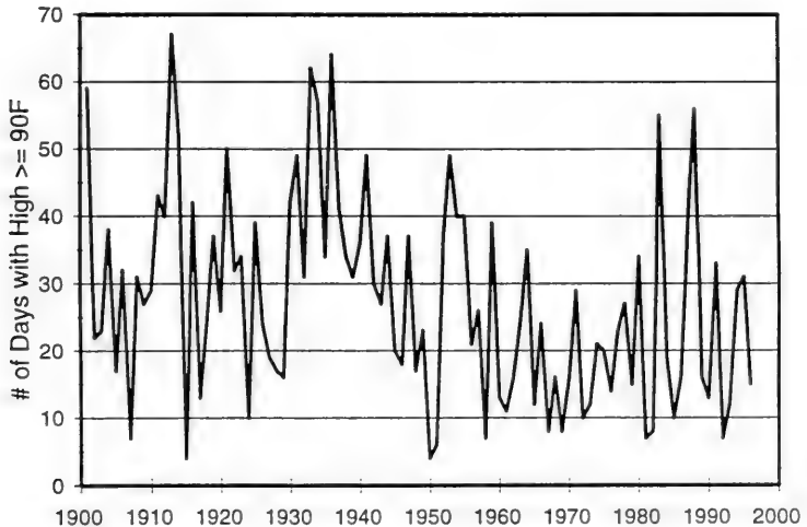
Figure 7. Annual Number of Days with Maximum Temperatures Equal to or Above 90°F at Peoria, 1901-1996
