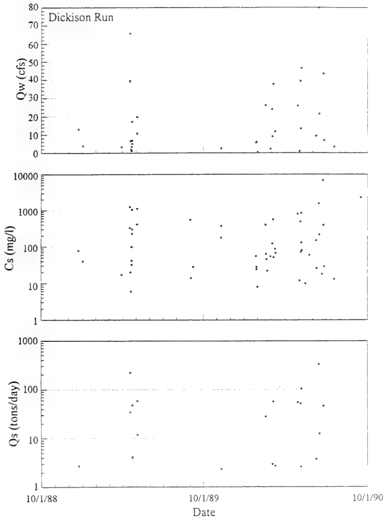
Figure 32. Variabilities of Flow Discharge and Instantaneous Suspended Sediment Concentration and Load for Dickison Run
