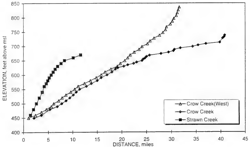
Figure 2. Stream Profiles for Three Tributaries in the Illinois River Bluffs Area
