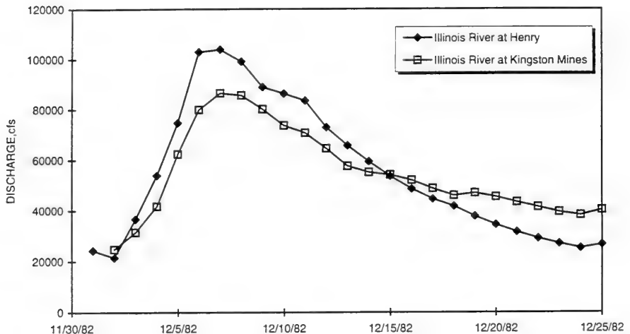
Figure 20. December 1982 Flood Hydrographs for the Illinois River at Henry and Kingston Mines
