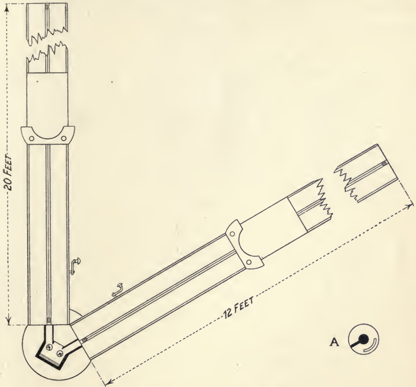
FIG. 56.—RUMFORD'S PHOTOMETER.
