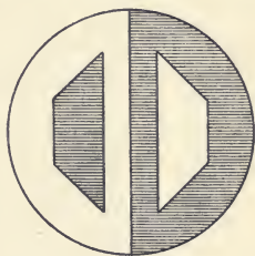
FIG. 74. — LUMMER-BRODHUN PHOTOMETER, CONTRAST FIELD OUT OF BALANCE.
