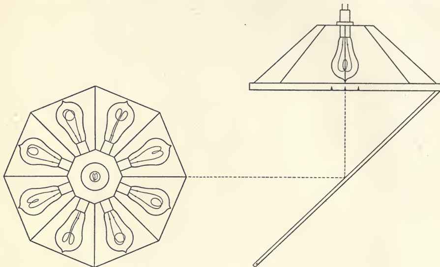
FIG. 101.—WILD'S MIRRORS FOR MEAN HORIZONTAL CANDLE-POWER.
