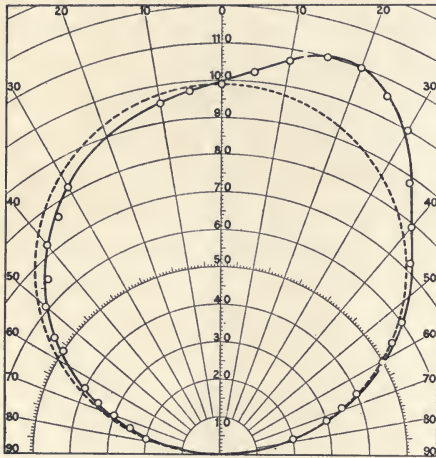
FIG. 147.—BADLY GLAZED SCREEN IN WORST POSITION.
