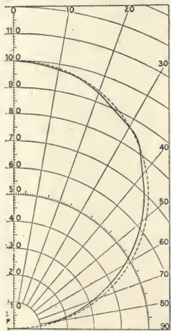
FIG. 165.—SHARP AND MILLAR TEST-PLATE ANGLE ERRORS.
