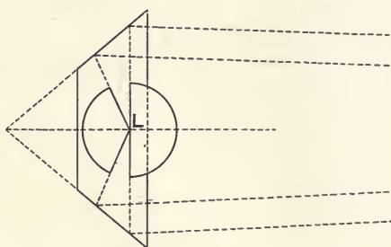
FIG. 115.—BLONDEL'S DIFFUSING CONE LUMENMETER.
