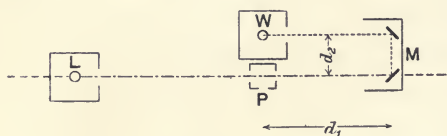
FIG. 91.—THE MOVING-MIRROR METHOD.
