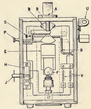
FIG. 158.—THE HARRISON PHOTOMETER, END VIEW OF INTERIOR.
