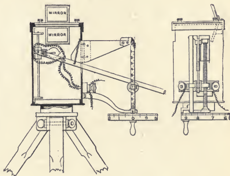
FIG. 135.—PREECE AND TROTTER ILLUMINATION PHOTOMETER.
