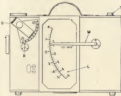
FIG. 157.—THE HARRISON PHOTOMETER, OUTSIDE VIEW.
