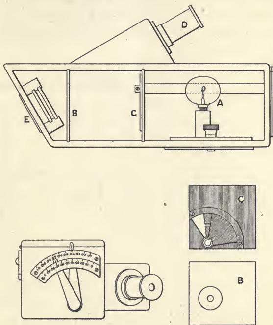
FIG. 168.—DOW AND MACKINNEY'S LUMETER.
