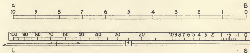
PHOTOMETER SCALE FIXED, POINTER MOVABLE.
