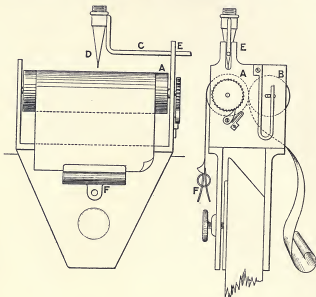
FIG. 95.—OBSERVATION RECORDER.
