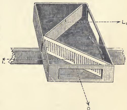
FIG. 81.—GRID PHOTOMETER.
