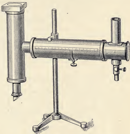
FIG. 160.—THE WEBER PHOTOMETER.
