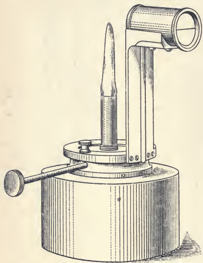
FIG. 2.—THE HEFNER AMYL-ACETATE LAMP.
