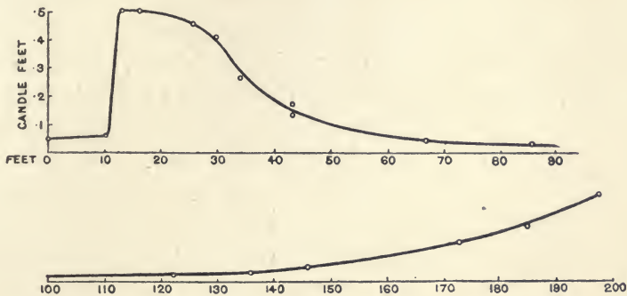
FIG. 172.—DISTRIBUTION OF ILLUMINATION AT CANNON STREET STATION (1872).
