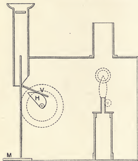
FIG. 166.—THE WINGEN-KRÜSS PHOTOMETER.
