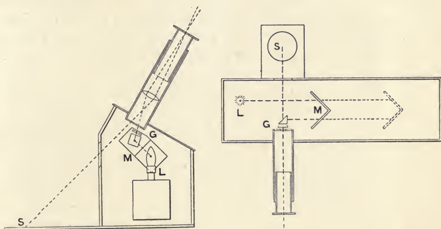
FIG. 167.—THE MARTENS PHOTOMETER. DIAGRAMMATIC PLAN, END VIEW.
