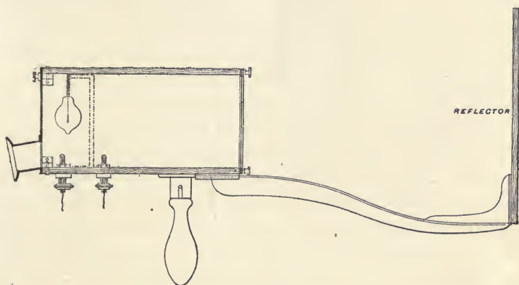
FIG. 134.—THE PREECE ILLUMINATION PHOTOMETER.
