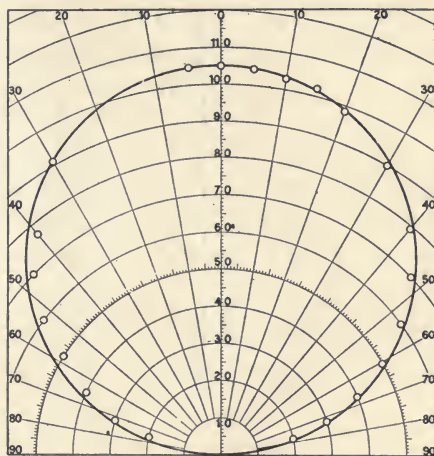
FIG. 149.—GOOD SCREEN IN WORST POSITION.
