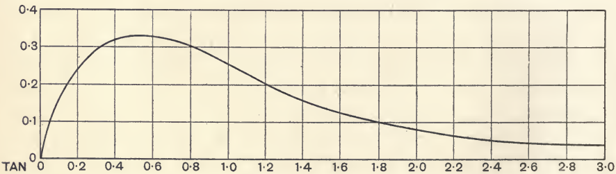
FIG. 16.—DISTRIBUTION OF ILLUMINATION FROM A VERTICAL FILAMENT.
