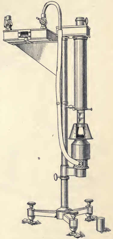
FIG. 1.—THE VERNON HARCOURT PENTANE 10-CANDLE LAMP.
