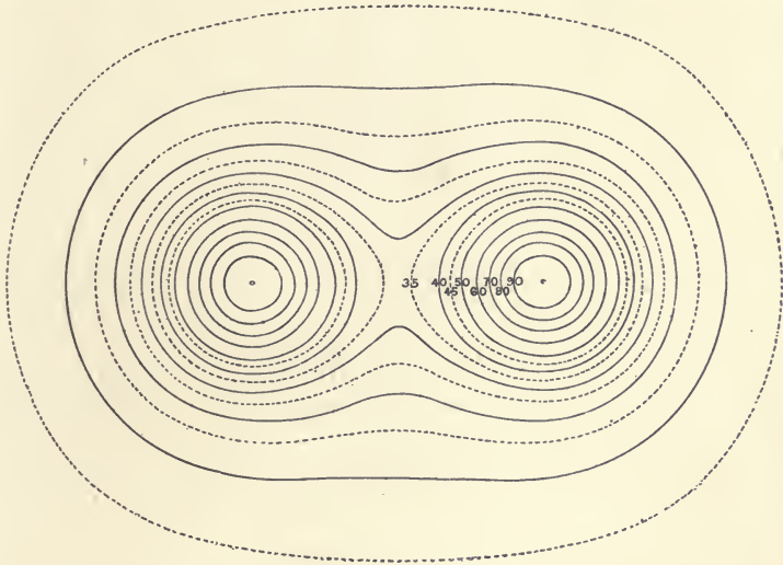
FIG. 27.—CONTOUR LINES OF EQUAL ILLUMINATION OR ISO-LUX CURVES, DUE TO TWO LIGHTS AT A DISTANCE APART EQUAL TO THREE TIMES THEIR HEIGHT.
