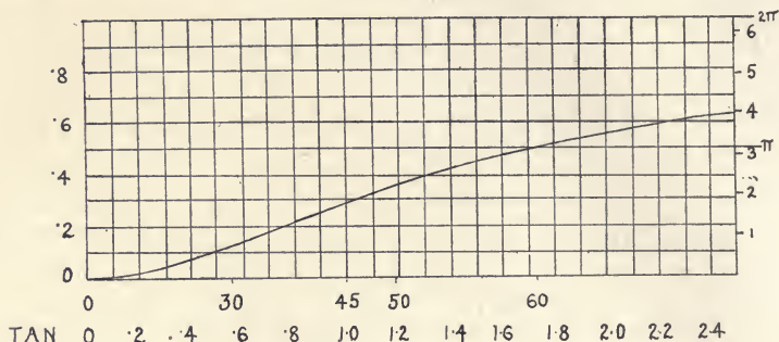
FIG. 40.—CURVE OF FLUX.
