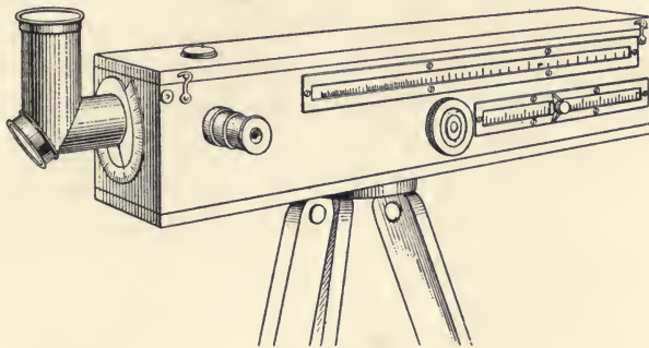
FIG. 162.—THE SHARP AND MILLAR PHOTOMETER.
