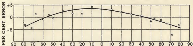
FIG. 151.—GOOD SCREEN IN BEST POSITION.
