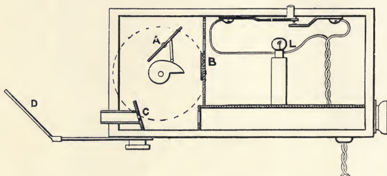
FIG. 169.—EVERETT-EDGCUMBE LUXOMETER.
