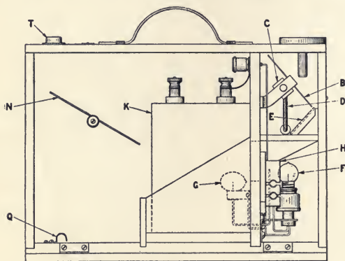
FIG. 159.—THE HARRISON PHOTOMETER, SIDE VIEW OF INTERIOR.
