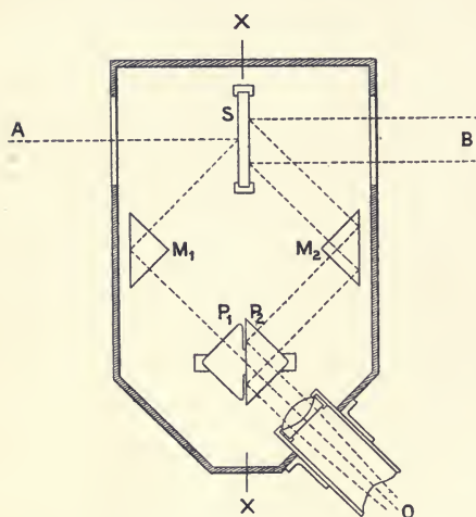
FIG. 73.—LUMMER-BRODHUN PHOTOMETER.
