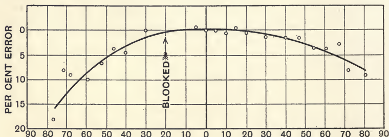
FIG. 150.—GOOD SCREEN IN WORST POSITION.
