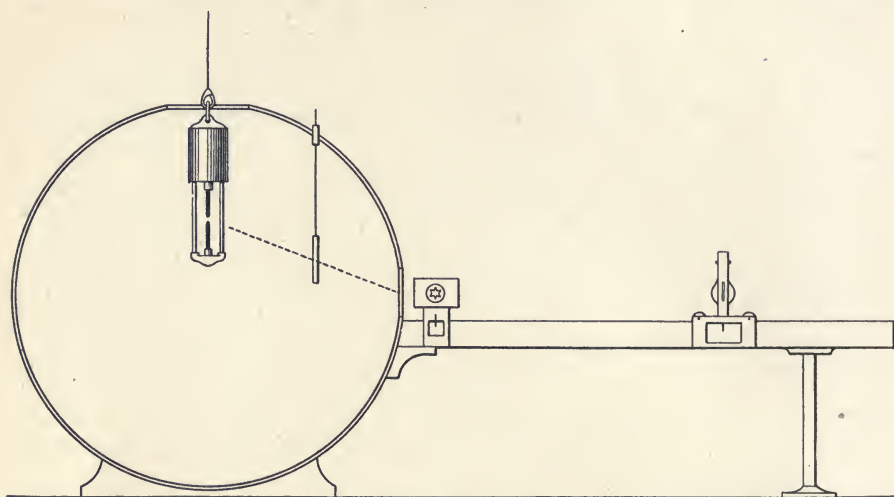
FIG. 120.—THE ULBRICHT GLOBE.
