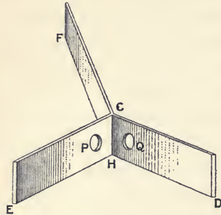
FIG. 55.—BOUGUER'S PHOTOMETER.
