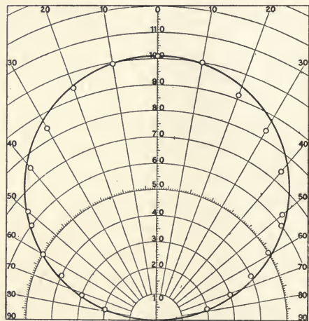
FIG. 148.—BADLY GLAZED SCREEN IN BEST POSITION.
