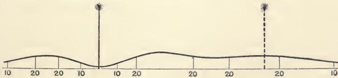
FIG. 35.—ILLUMINATION CURVE ALONG THE LINE AB, FIG. 34.
