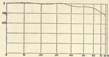
FIG. 164.—SHARP AND MILLAR TEST-PLATE ANGLE ERRORS.
