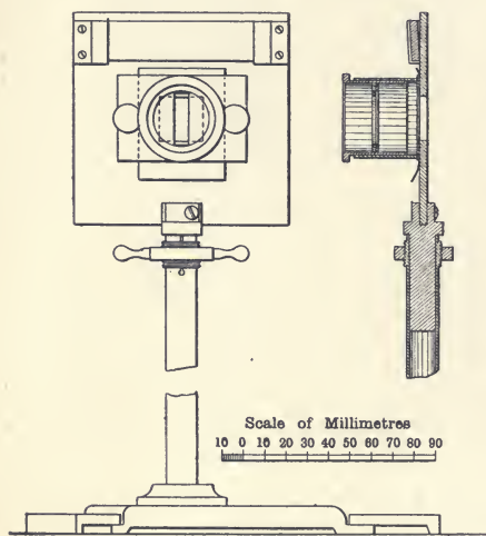
FIG. 58.—THE VERNON HARCOURT GAS REFEREES' PHOTOMETER.
