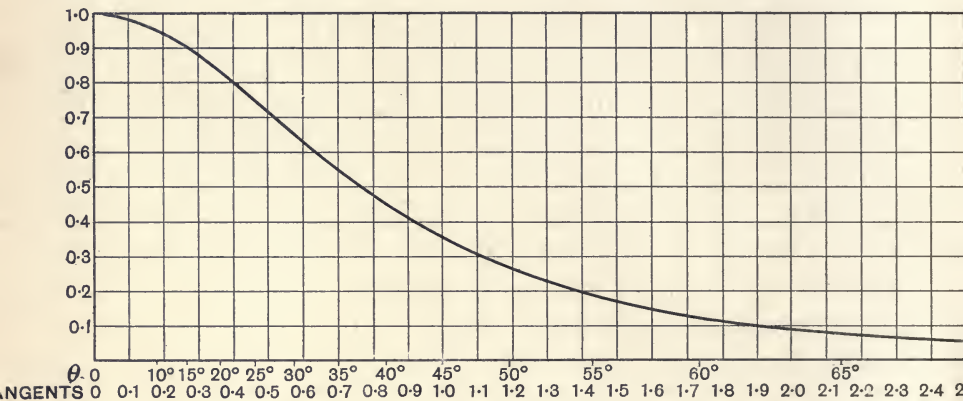
FIG. 9.—CURVE OF COSINES CUBED.
