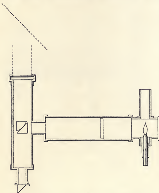
FIG. 161.—THE WEBER PHOTOMETER SECTION.
