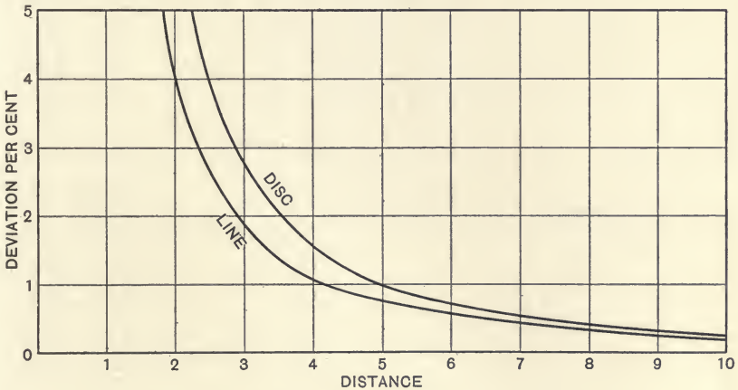
FIG. 90.—DEVIATION FROM THE LAW OF INVERSE SQUARES.
