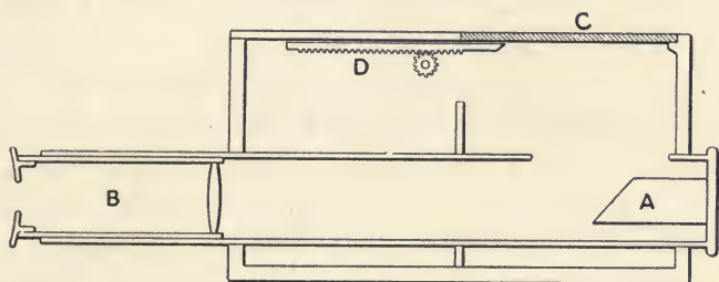
FIG. 53.—HOUSTON AND KENNELLY'S PHOTOMETER.
