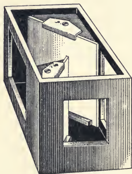
FIG. 71.—THE CONROY PHOTOMETER, PERSPECTIVE VIEW.
