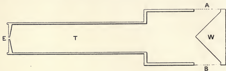
FIG. 54.—FLEMING'S DISCRIMINATION PHOTOMETER.
