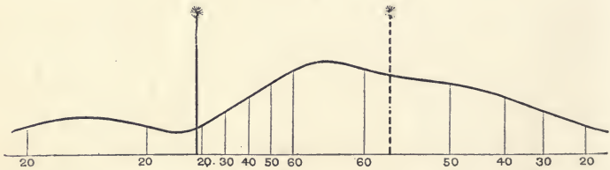
FIG. 33.—ILLUMINATION CURVE ALONG THE LINE AB, FIG. 32.
