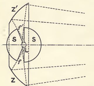
FIG. 114.—BLONDEL'S ANNULAR ELLIPSOIDAL LUMENMETER.
