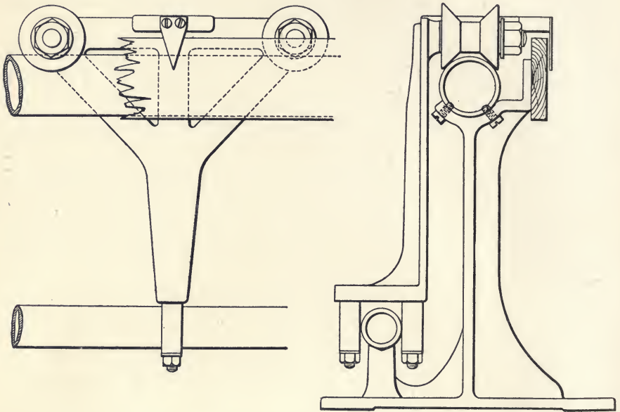
FIG. 92.—EVERETT-EDGCUMBE PHOTOMETER BAR AND CARRIAGE.
