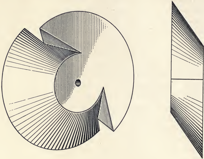
FIG. 126.—WHITMAN'S DISC FOR FLICKER PHOTOMETER.
