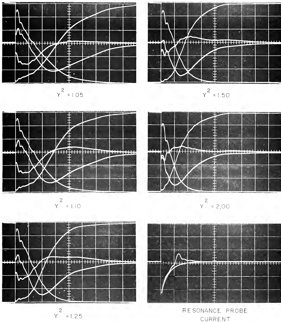
Figure 4.1.6b Slotted line voltage as a function of time. (Neon at 4.3 mm. pressure. Time scale: 320 \mu\text{s}/\text{cm}. )
