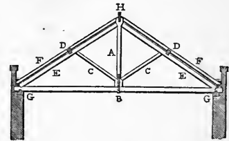
King Post Roof.
