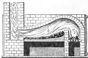
Reverberatory Furnace.
