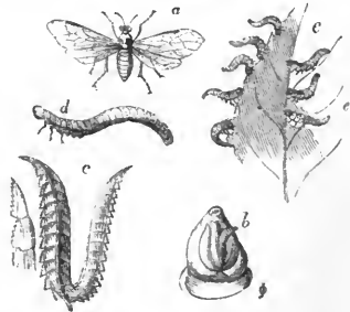
Tenthredo, Saw-fly.
