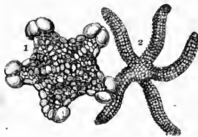
Star-Fish.
