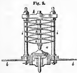
Spring Safety-valve.
