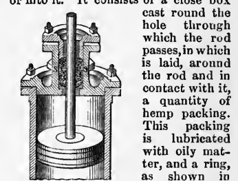
Part of Steam-engine Cylinder. s, s, Stuffing-box.
