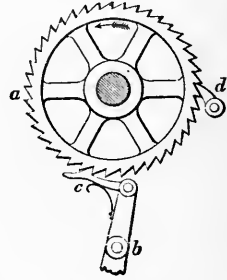
Rätchet-Wheel.
