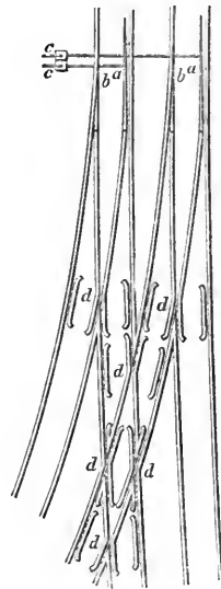
Junction Rails.
