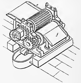
Horizontal Sugar Mill.
