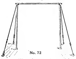
No. 72. Wrought iron pipe uprights, detachable iron head pieces, steel guy wires, wrought iron turnbuckles and floor plates; steel core bar.
