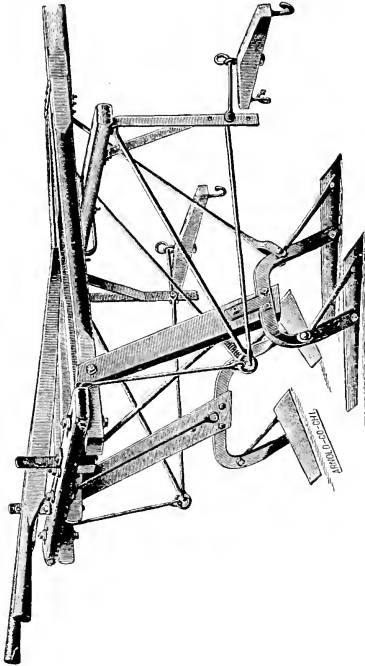
FIG. 22.—BRADLEY GOPHER CULTIVATOR.
