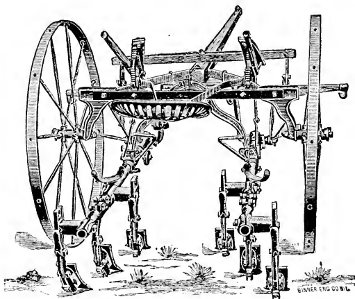
FIG. 21.—STANDARD RIDING CULTIVATOR WITH SIX SHOVELS.
