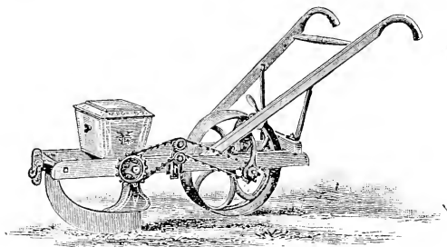
FIG. 26.—FARMERS' FAVORITE ONE-HORSE CORN DRILL.
