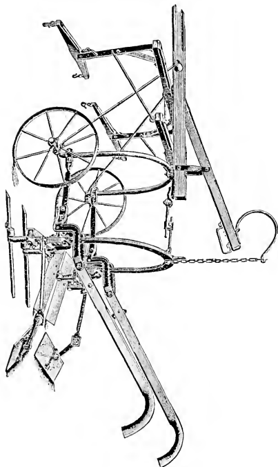
FIG. 24.—TOWER CORN CULTIVATOR.
