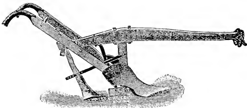
FIG. 30.—LISTING PLOW.
