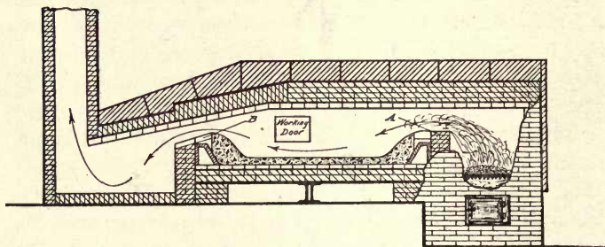
FIG. 40. Puddling Furnace.
