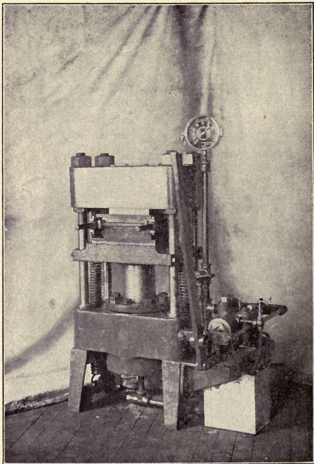
FIG. 26. Hydraulic Press.
