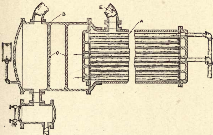
FIG. 18. Section through a Yaryan Evaporator.
