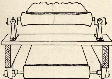
FIG. 7. Supports for Belt Conveyor.
