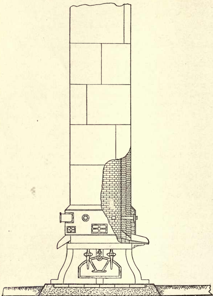
FIG. 39. Foundry cupola.
