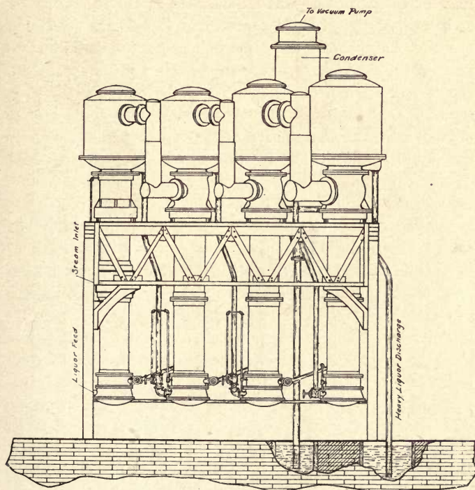
FIG. 21. Kestner Climbing Film Evaporator.
