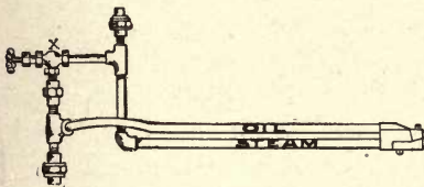
FIG. 35. Commercial Type of Fuel Oil Burner.
