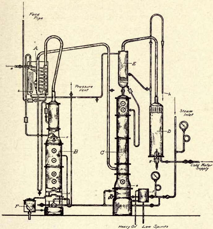
FIG. 22. Continuous Column Still.
