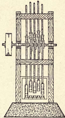
FIG. 9. Stamp Mill.
