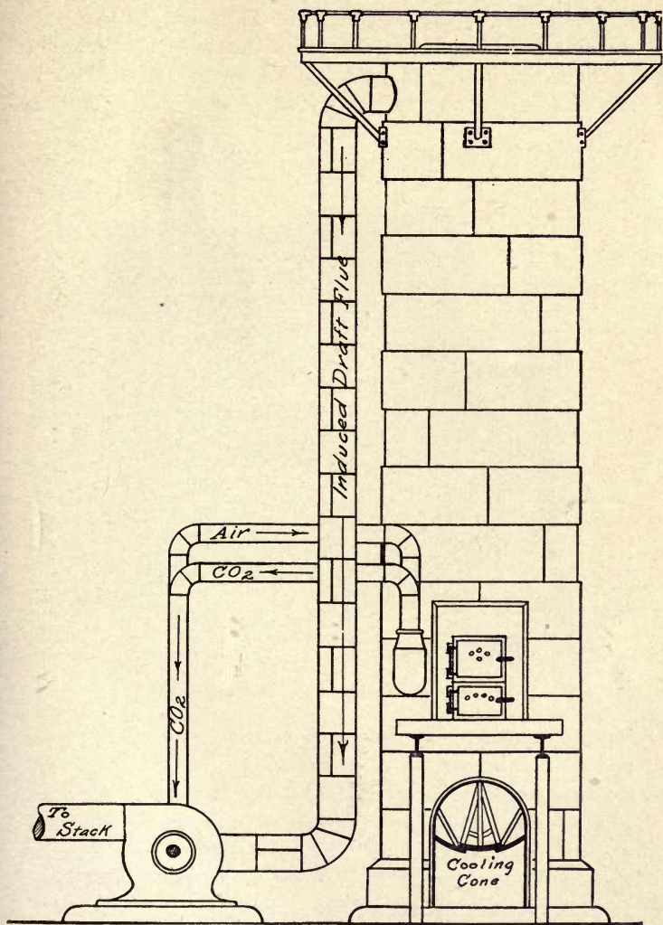
FIG. 48. Modern Type of Lime Kiln.
