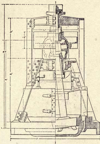
FIG. 13. Griffin Mill (of slightly different design)—Section.
