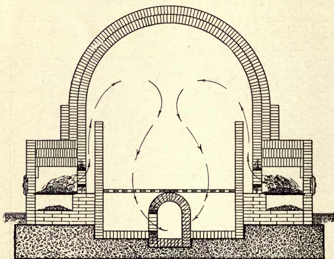
FIG. 45. Down-Draft Brick Kiln.
