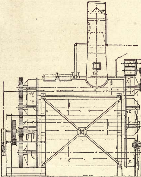
FIG. 50. Section through Kritzer Lime Hydrator (arrows show the course of the lime during hydration).
