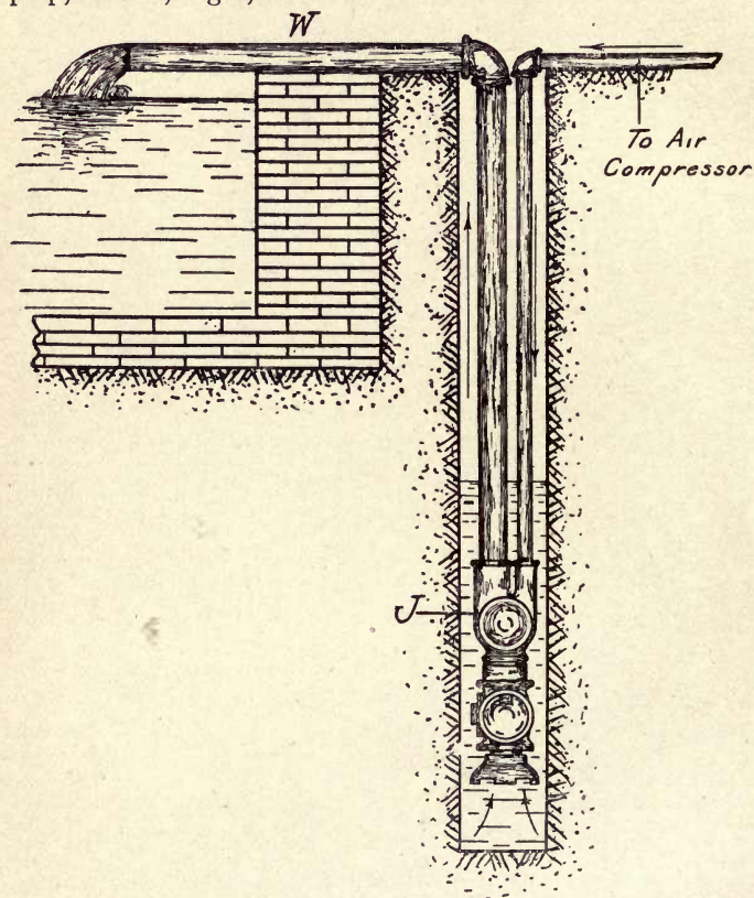
FIG. 4. Air Jet Lift.
