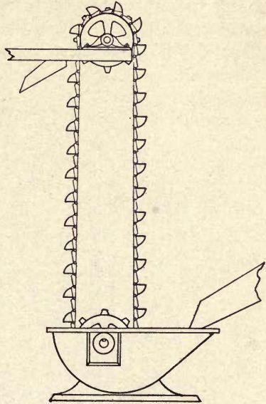
FIG. 6. Bucket Elevator.
