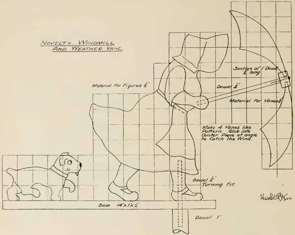
WINDMILL DRAWING CONTRIBUTED BY HAROLD R. WISE, PROVIDENCE, R. I.
