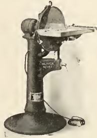
"Oliver" No. 182 Disk Sander
