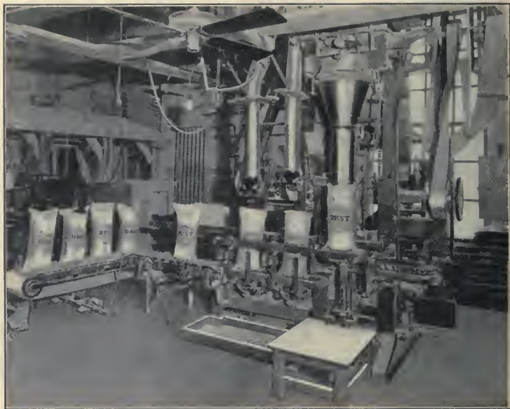
GIANT FLOUR-PACKING MACHINE, AUTOMATICALLY FILLING, WEIGHING, AND SEWING FLOUR SACKS
