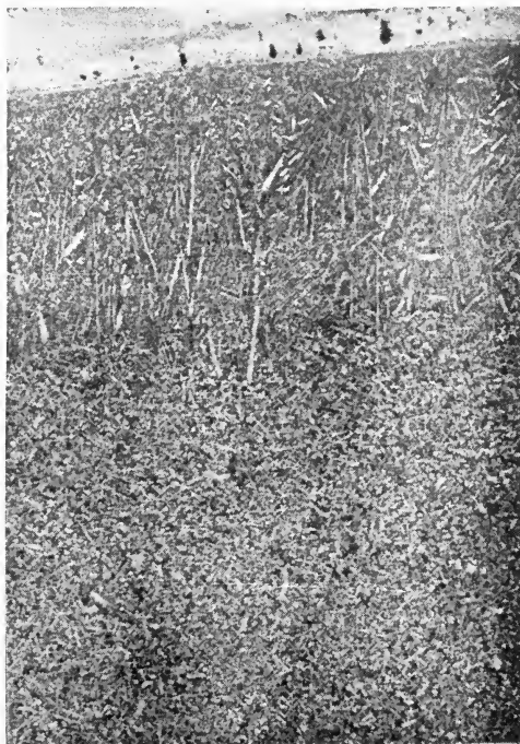
FIG. 73.—Sulphur print of top-poured ingot.
