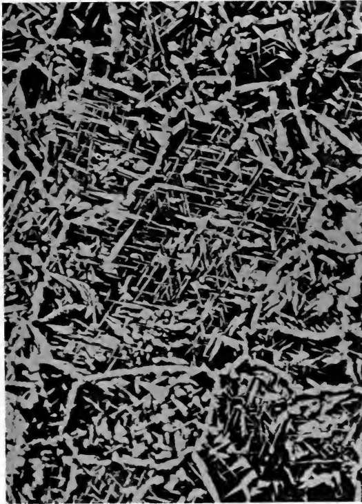
FIG. 63.—Re-heated ingot or billet structure \times 25 .
