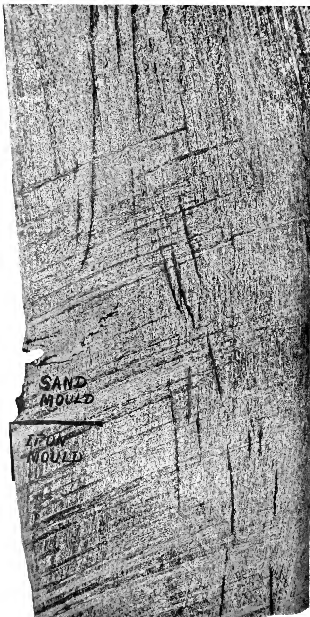
FIG. 82.—Ghosts in large ingot (Ashdown).
