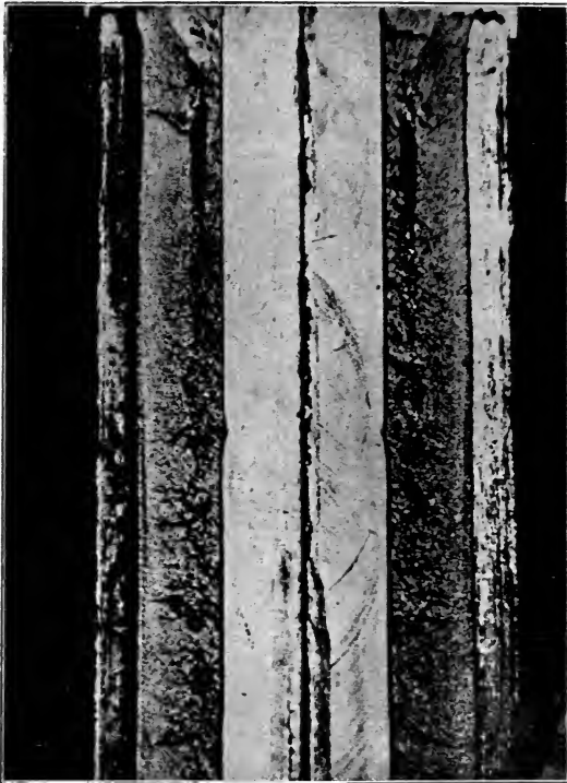
FIG. 31a.—Cavities below dozzle in crucible ingots.
