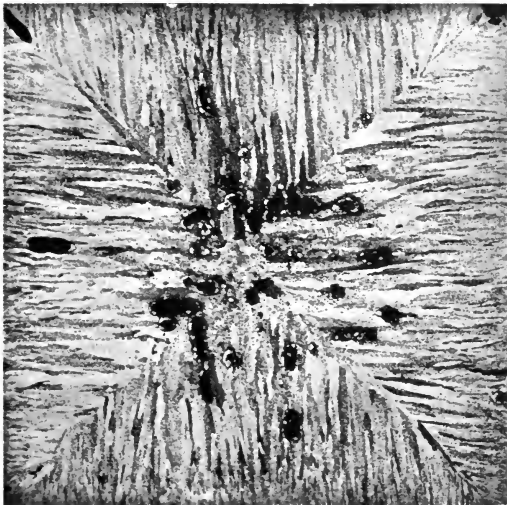
FIG. 15.—Cracked surfaces corroded by pickling.
