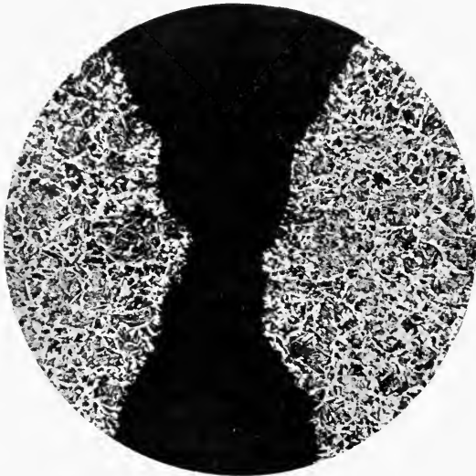
FIG. 41.—Structure of material about bright cavities \times 16 .
