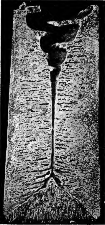
FIG. 12.—Diagonal contraction cavities.
