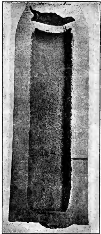
FIG. 11.—Open-hearth ingot intentionally bled.
