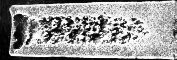
FIG. 72.—Relative rate of freezing of "wild" and sound wax ingots.
