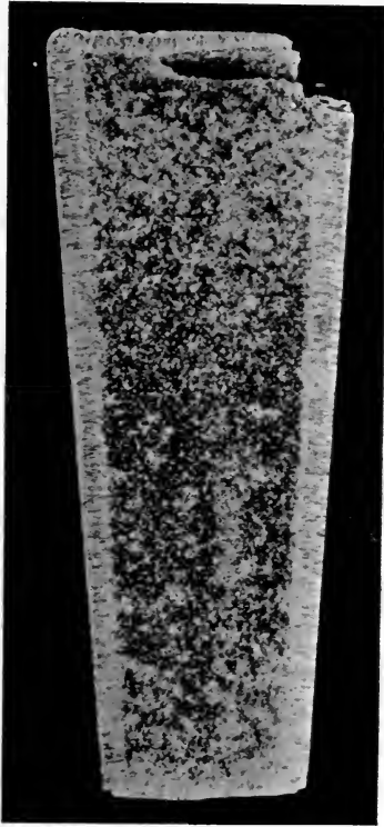
FIG. 21.—Deposited free crystals in solid wax ingot.
