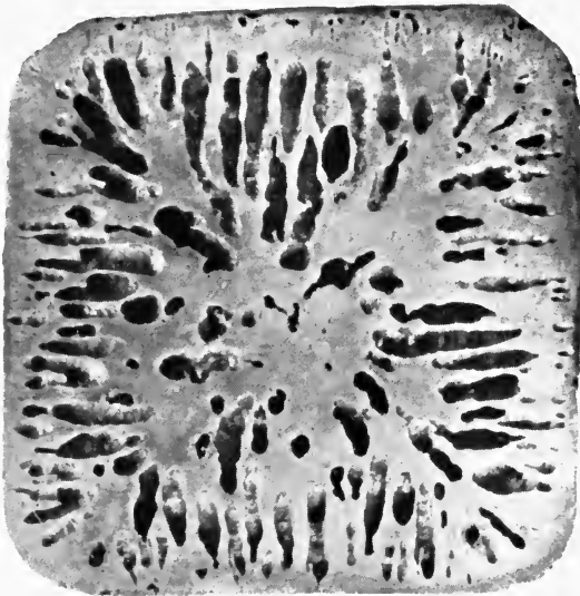
FIG. 75.—Blow-holes caused by rusty moulds.
