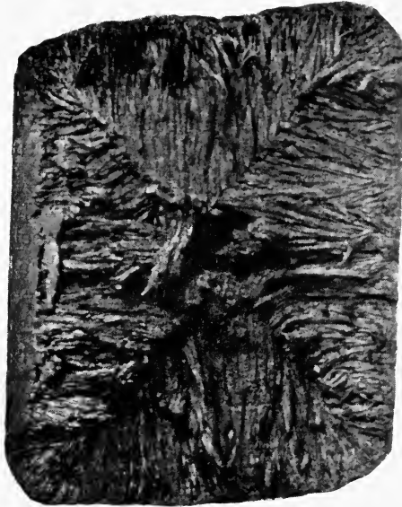
FIG. 26.—Fracture of "hot-cast" nickel steel ingot.
