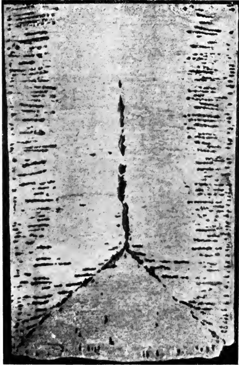
FIG. 99.—Ingot section, showing cavities on base pyramid.
