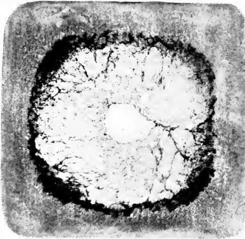
FIG. 80.—Sulphur print of Talbot billet—transverse section.
