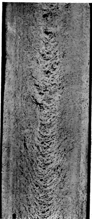
FIG. 54.—Shrinkage depressions in German silver ingot.
