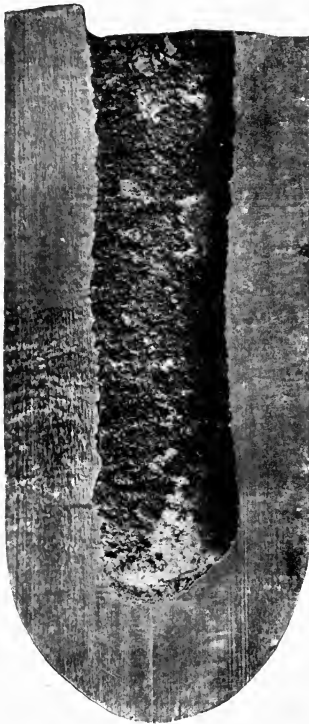
FIG. 10.—Partly fluid crucible ingot intentionally inverted.
