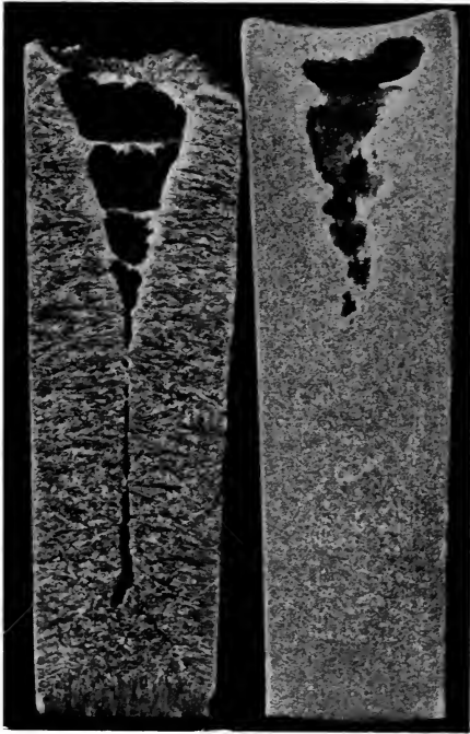
FIG. 33.—Relative shrinkage and contraction in hot- and cold-cast ingots.
