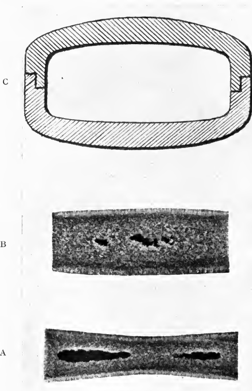
FIG. 36.—Sections of flat ingot and mould.
