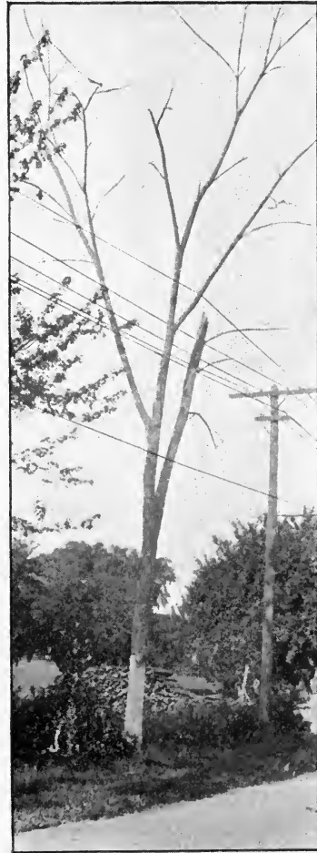
Fig. 7. Maple tree killed by direct current from a trolley system, carrying positive current through the rail, and return current through the feed wire in contact with branches. The largest amount of burning occurred slightly remote from the point opposite the rail, and in line with a large root, lying diagonally with, and just under the nearest rail.
