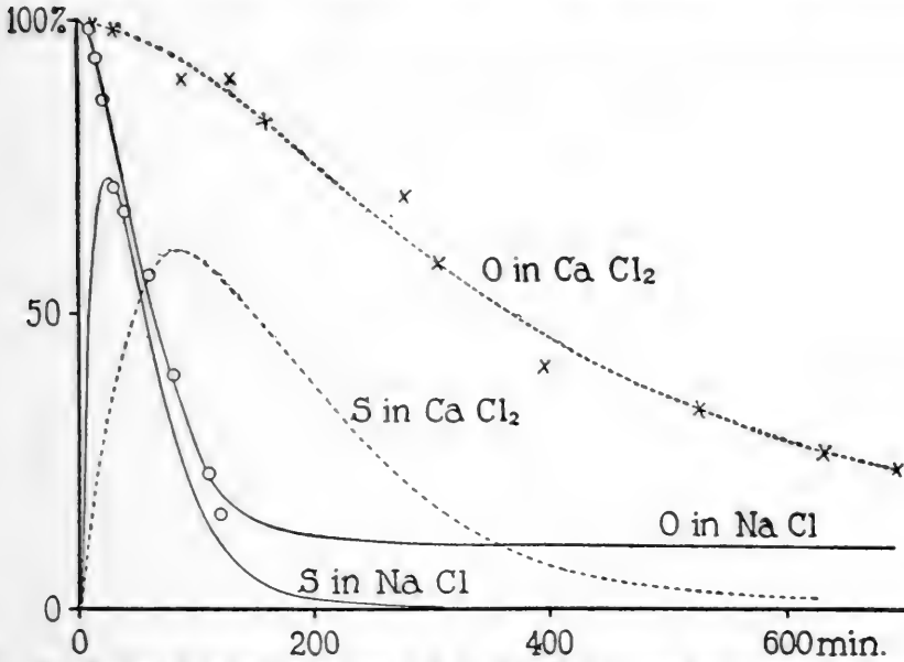
FIG. 43.—Curves showing the values of O + 10 in NaCl (upper unbroken line) and in CaCl (upper dotted line); also the values of S in NaCl (lower unbroken line) and in CaCl 2 (lower dotted line). The ordinates give the values of O ; these must be multiplied by 6.75 to obtain the values of S . The observed points represent the average of eight or more experiments; probable error of the mean less than 10% of the mean.
