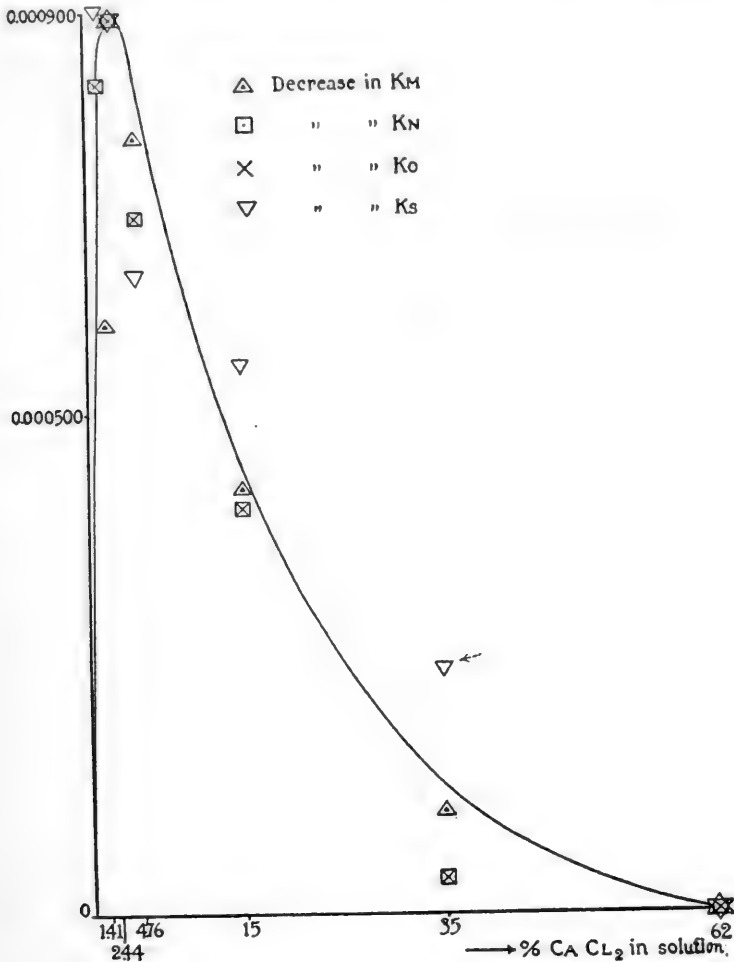
FIG. 64.—Shows the increase of a hypothetical salt compound Na_4XC_2 (see Table XI) and the corresponding decrease of the velocity constants K_N , K_O , K_S and K_M (these constants are given in Table X). The figures on the abscissæ give the molecular per cent. of CaCl_2 in the mixture. The mixture containing 62.0% CaCl_2 is taken as the standard of comparison: proceeding from this to the mixtures containing less CaCl_2 we find that Na_4XC_2 increases and the velocity constants decrease as shown by the ordinates. In order to facilitate comparison the values of K_N have been multiplied by 0.989; of K_O by 0.991; of K_S by 0.383; and of K_M by 0.251.
