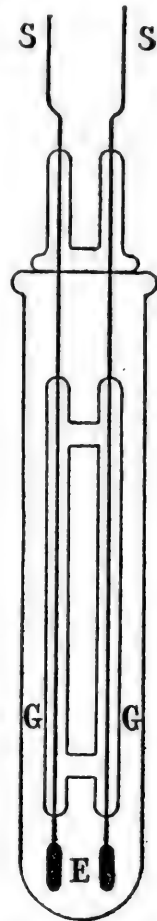
FIG. 2.—Apparatus for measuring the electrical conductivity of sea urchin eggs (Gray): S , silver wires, G, G , glass tubes; E , platinum electrodes.
