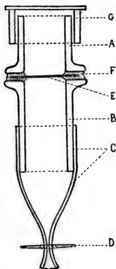
Fig. 89.—Apparatus for testing the rate of diffusion of salts through living tissue. It consists of two glass cells A and B (the former is provided with a cover, G ) separated by a layer of living tissue of Laminaria , E , which is sealed to the glass cells by a mixture of vaseline and beeswax, F . The lower cell is provided with a piece of rubber tubing, C , and a pinch cock, D .
