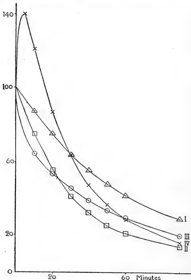
FIG. 32.—Curves showing the value of M when the velocity constants have the values given below.
