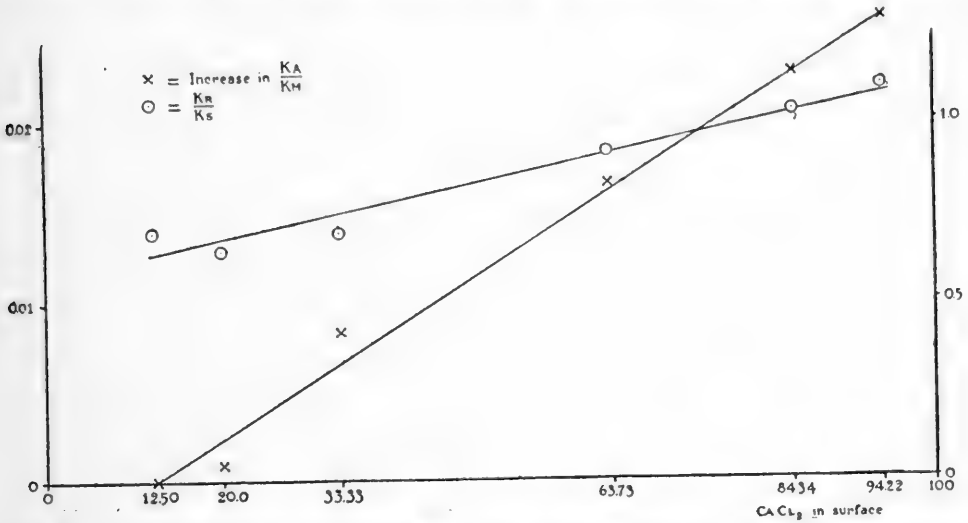
FIG. 65.—Graph showing the increase of K_A \div K_M and the value of K_R \div K_S as the molecular per cent. of \text{CaCl}_2 increases. The figure shows that \text{CaCl}_2 acts as a catalyzer of the reaction A \rightarrow M (which has the velocity constant K_A ) and also of the reaction R \rightarrow S (which has the velocity constant K_R ). The figures on the ordinate at the right show the values of K_R \div K_S ; those on the ordinate at the left show the increase in the value of K_A \div K_M over the value found in the mixture containing 1.41% \text{CaCl}_2 . The abscissæ denote molecular per cent. of \text{CaCl}_2 in the surface (not in the solution).
