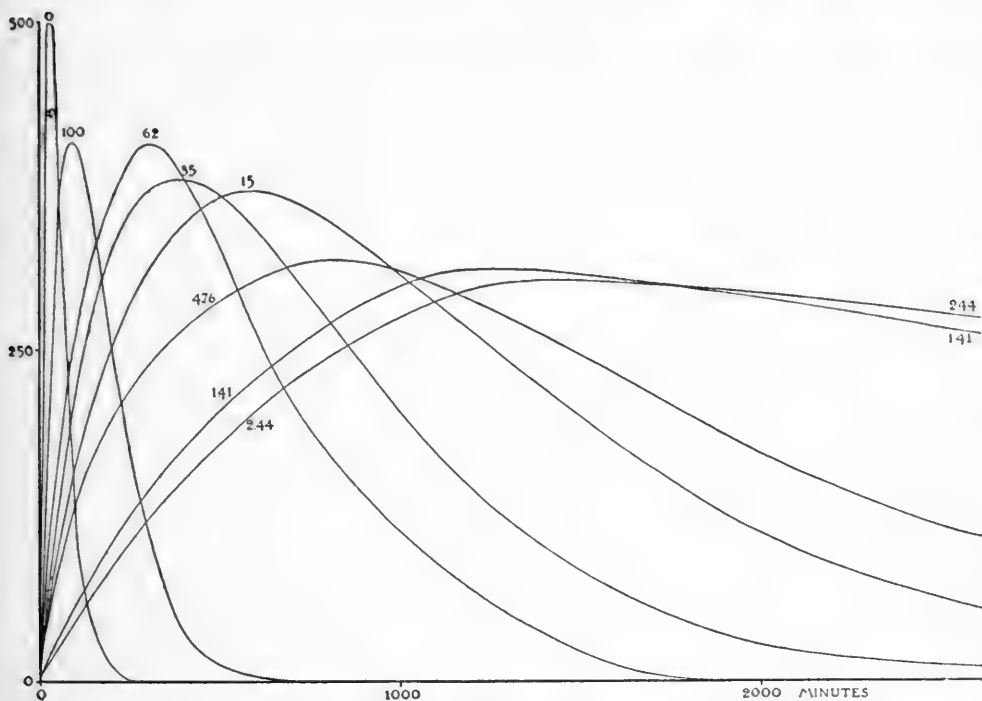
FIG. 67.—Curves showing the (calculated) values of S in 0.52 M NaCl, 0.278 M CaCl 2 , and in mixtures of these (the figures attached to the curves show the molecular per cent. of CaCl 2 in the solution). The curves show the values calculated from constants obtained by trial which are given in Table X. The abscissæ represent the time of exposure to the toxic solution. The value of S at the start is in all cases 2.7.
