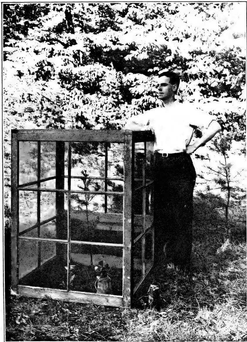
FUMIGATION CHAMBER FOR TESTING EFFECTS OF SULPHUR DIOXID ON YOUNG TREES.
