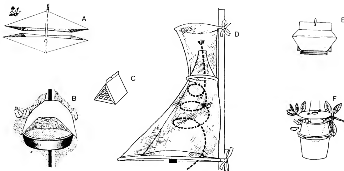
Figure 2. Commercially available traps used for monitoring insect populations include (A) the "wing" trap; (B) the water pan trap; (C) the Delta trap; (D) the Heliiothis trap; (E) the Pherocon II trap; and (F) the funnel trap. Several other trap designs also are available.
