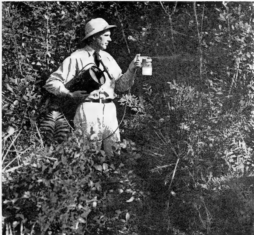
FIGURE 4.—Outdoor spraying with a DeVilbiss paint sprayer.
