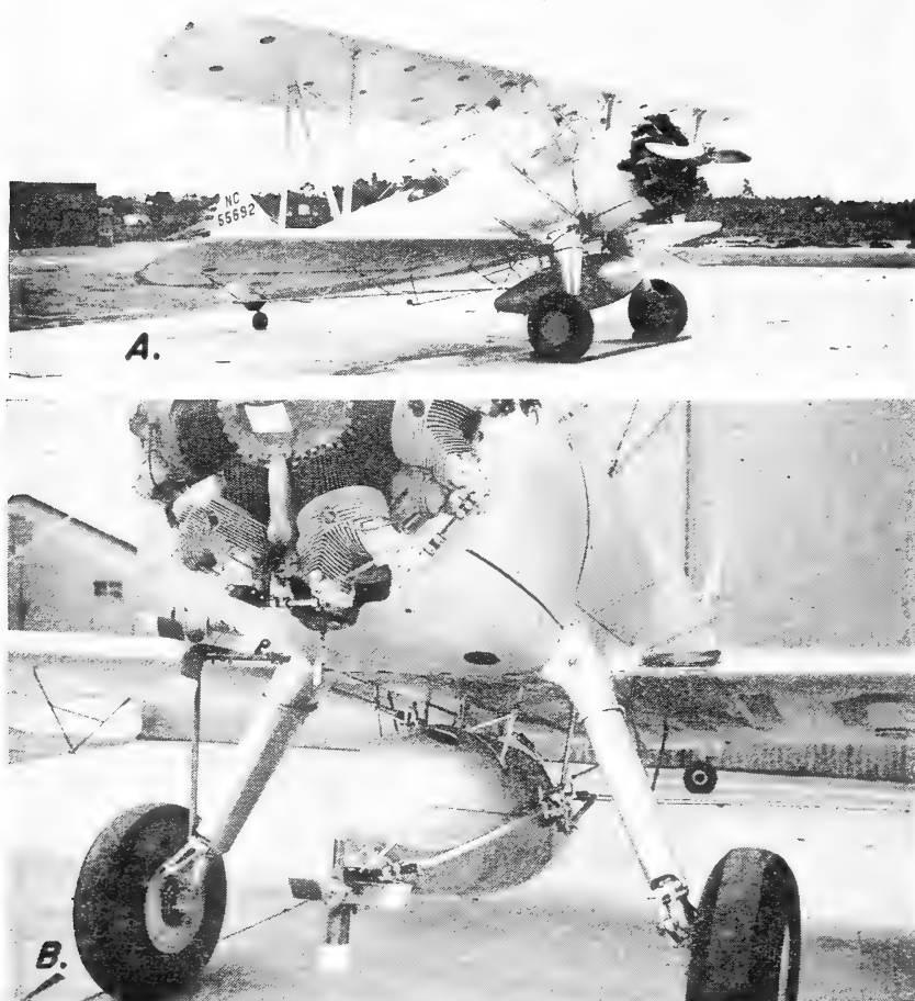
FIGURE 17.—A PT-17 plane with belly tank installed: A , Wind-driven gear pump mounted on landing-gear strut; B , wind-driven rotary pump mounted in front of tank for use with suspensions.
