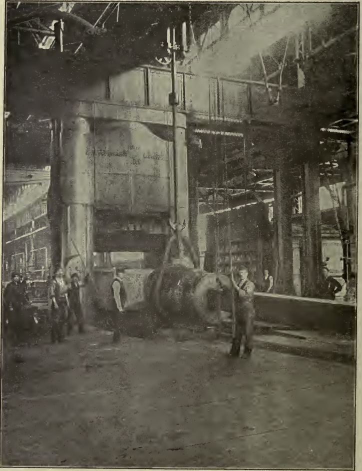
Huge ingot being forged for armor-plate under the 12,000-ton hydraulic press at Homestead.
