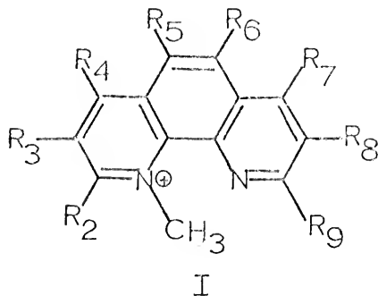
Figure 18. The N-Methyl-1,10-Phenanthrolium Cation.
