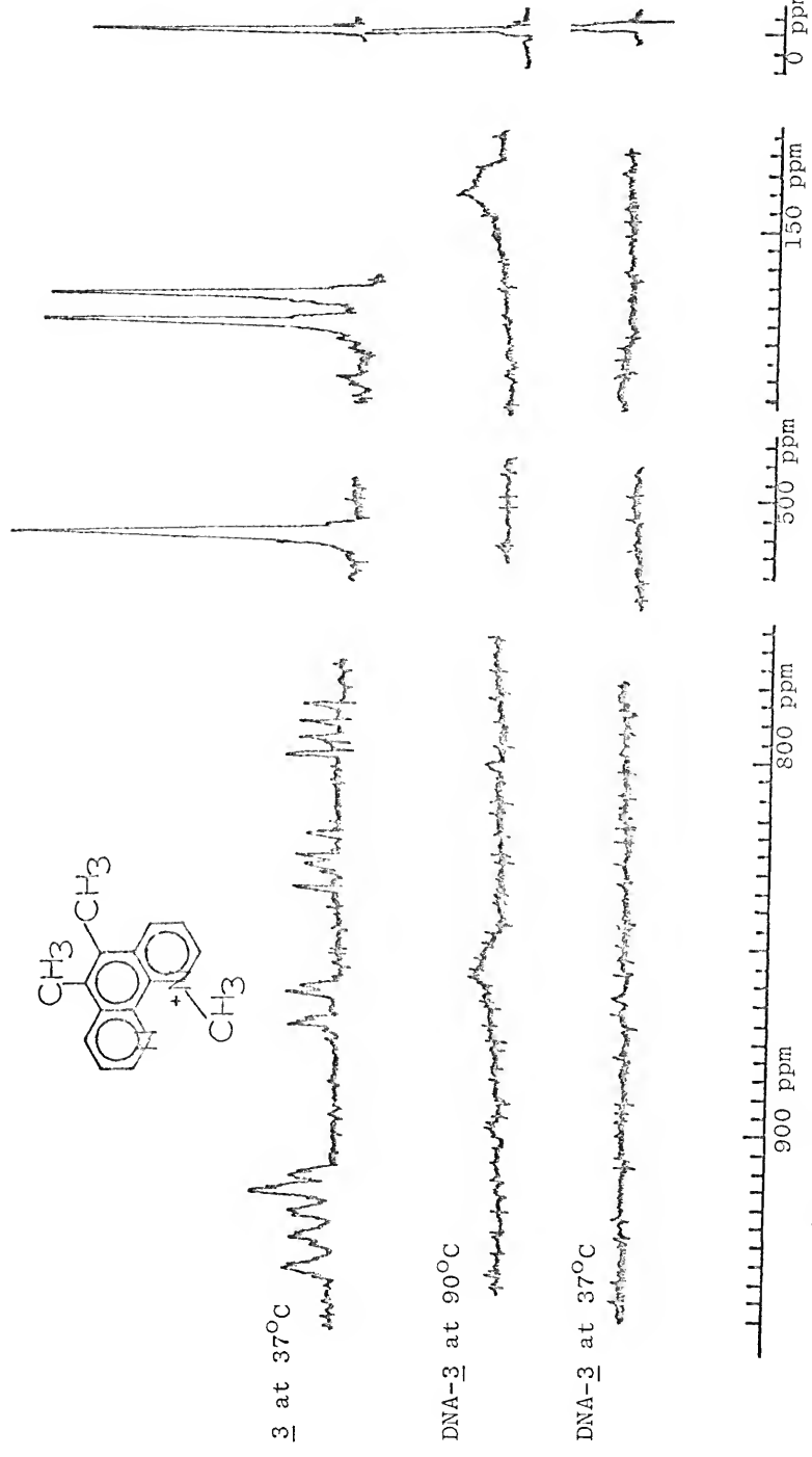
Figure 19. The Temperature-Dependent Partial Proton Magnetic Resonance Spectra of 3 and Salmon Sperm DNA- 3 Complex. Sonicated low molecular weight salmon sperm DNA was used at 0.15 mole of P/1 in D 2 O in 10 -4 sodium phosphate buffer (pD 7.0± 0.2). The concentration of 3 was 0.02 M.
