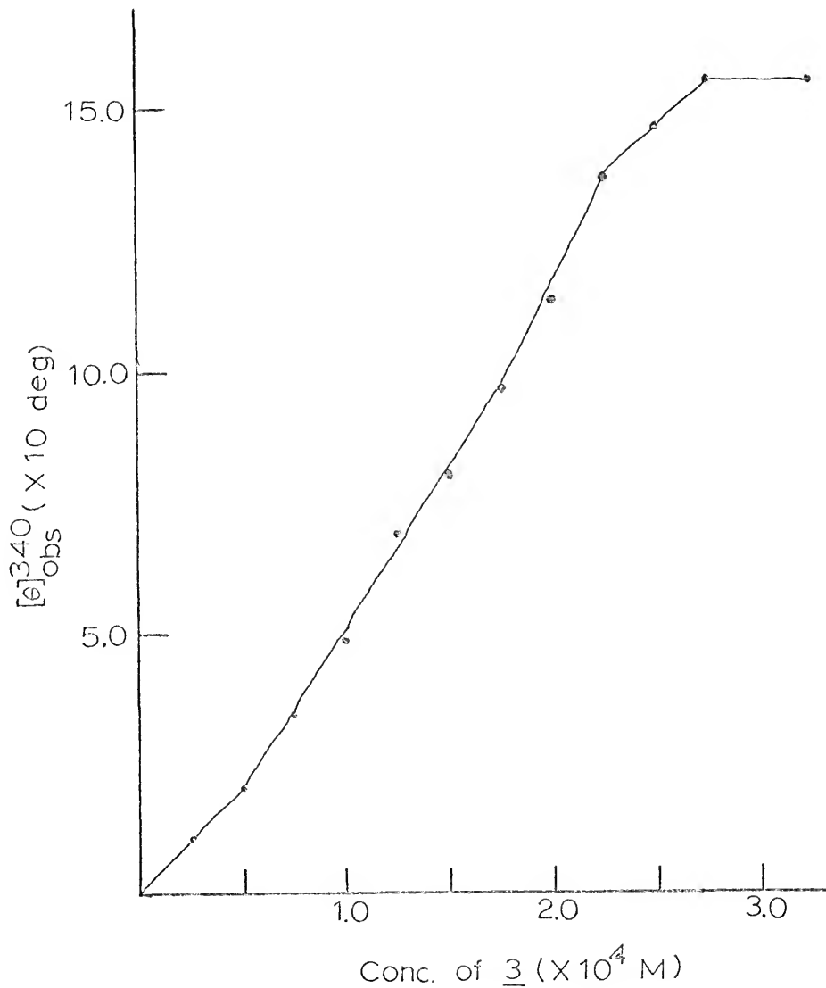
Figure 22. The Effect of Increasing Concentration of \underline{3} on the Observed Ellipticity, (\theta)_{\text{obs}} , at 340 nm in the Presence of 5.60 \times 10^{-4} M P/1 of Salmon Sperm DNA.
