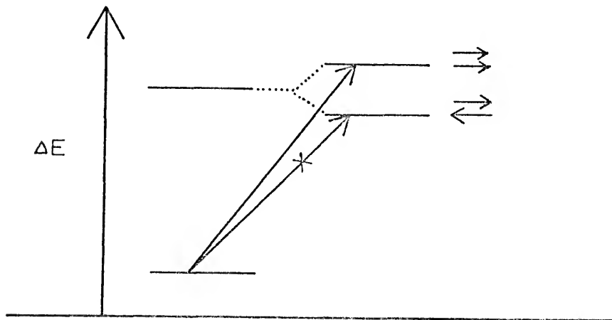
Figure 12. Exciton Splitting of the Energy Levels.
