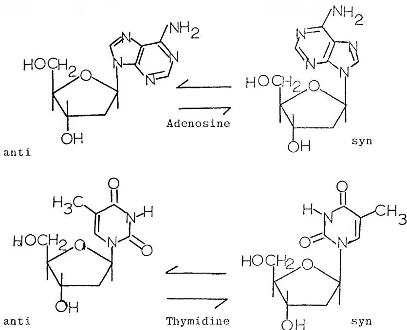
Figure 11. The Anti and Syn Conformations of a Purine and Pyrimidine Nucleoside.
