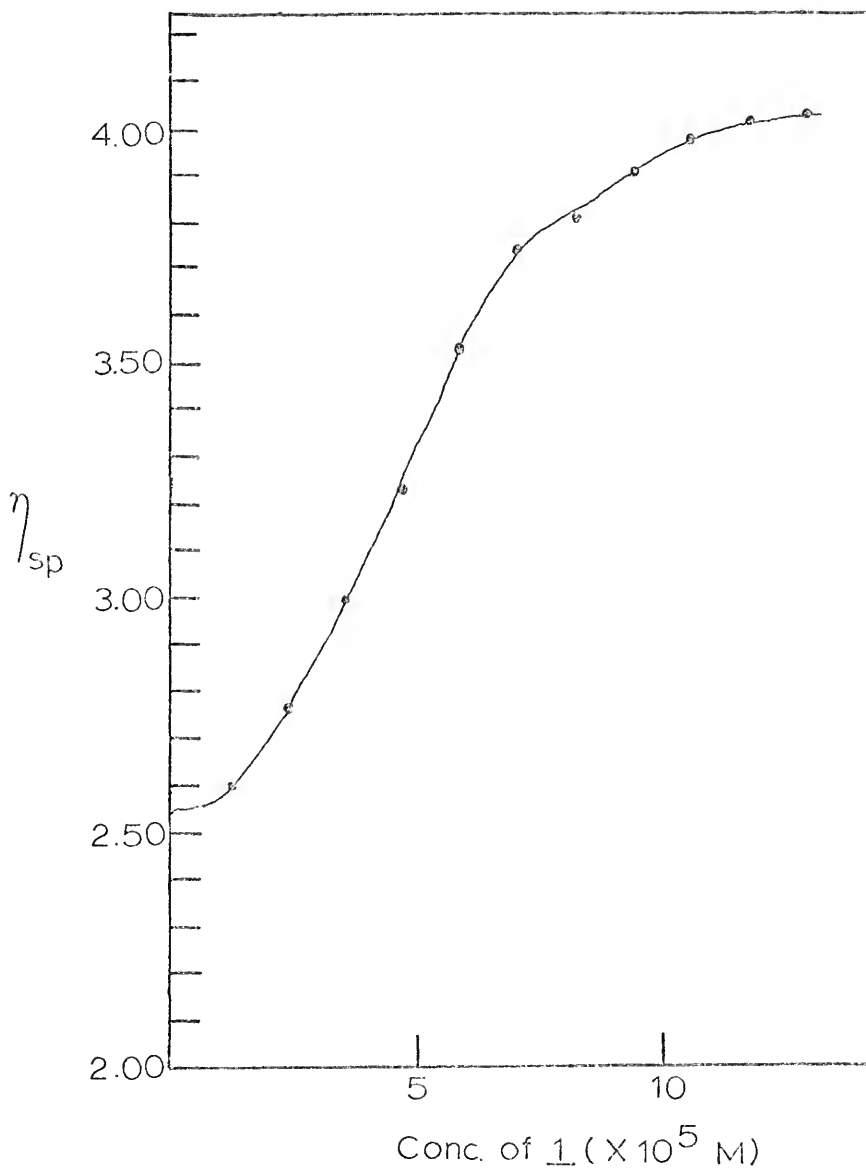
Figure 29. The Effect of Increasing Concentrations of [bar] on the Relative Specific Viscosity. The study was conducted in 0.01 M MES buffer, pH 6.2 (0.005 M \text{Na}^+ ) at 37.5^\circ\text{C} using 5.60 \times 10^{-4} M P/l of salmon sperm DNA.
