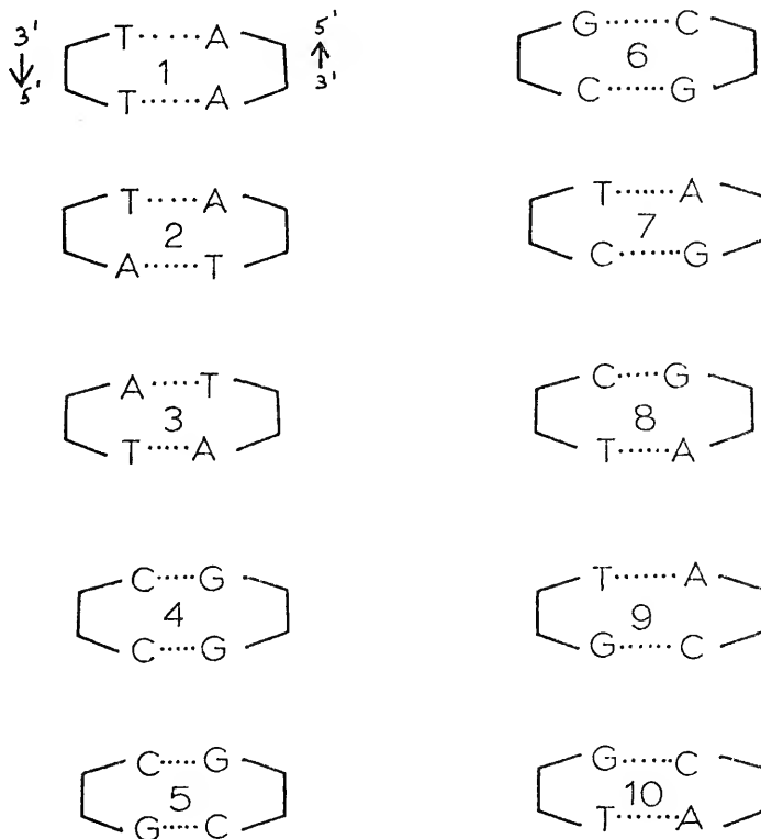
Figure 13. The Ten Different Intercalating Sites in DNA.
