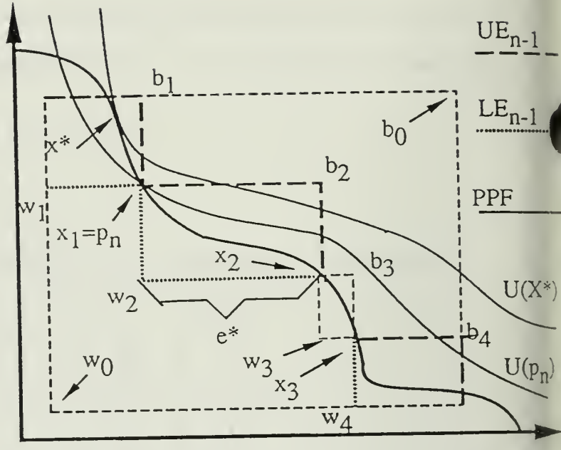
3b) Steps 2 and 3: b_2 is found to be inferior to p_n and so b_2, w_2, and c_2 are discarded.
