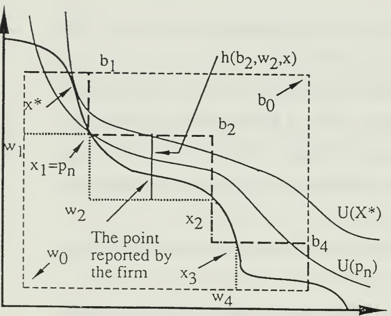
3c) Step 4: The x th edge of the second cube is found to be the longest. Case 1 holds and the firm reports a point in the intersection of h(b_2, w_2, x) and the PPF.
