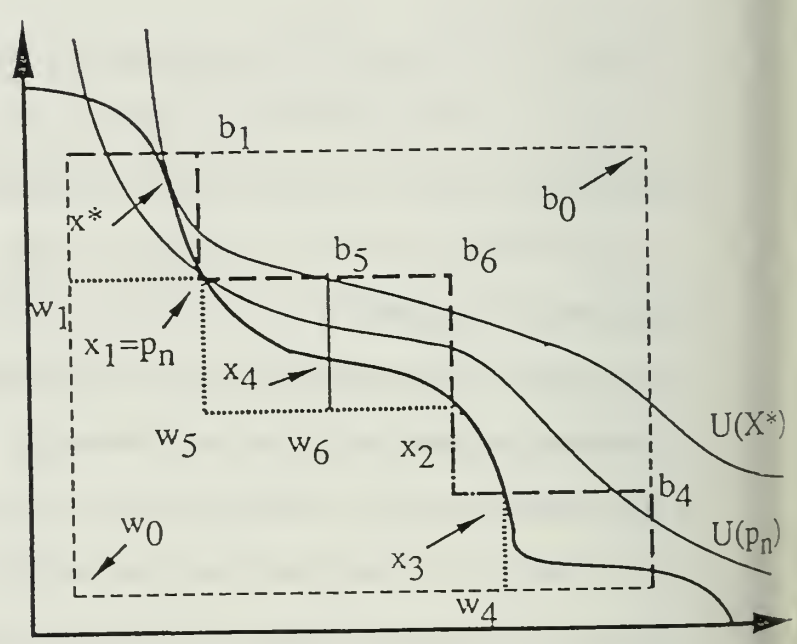
3d) Step 5: c_2 is divided in two along the x axis and replaced with the two new cubes, and appropriate best and worst points.
