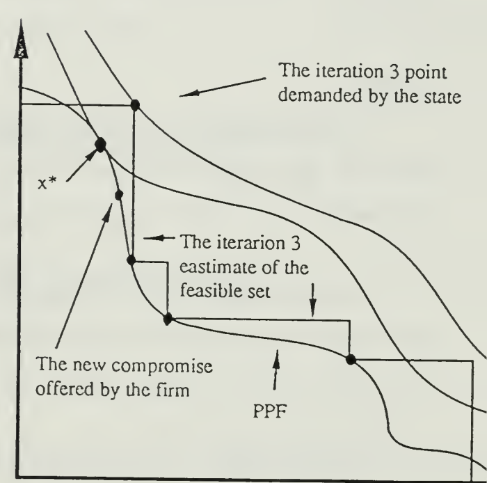
1d) Iteration 3
