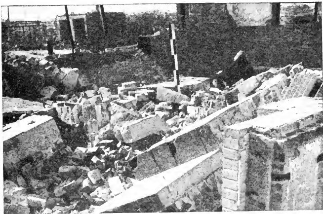
FIGURE 4.— Upper photo: Building with load-bearing walls, 5,200 feet from ground zero. Load-bearing wall away from the blast collapsed. Lower photo: Interior of same building, showing damage from blast and fire.
