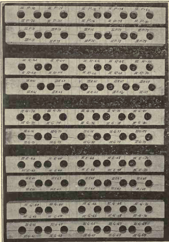
PLATE 8.—Laminated maple showing tension failures due to moisture difference at time of gluing. Odd numbers indicate glued pieces. Even numbers indicate free pieces.
