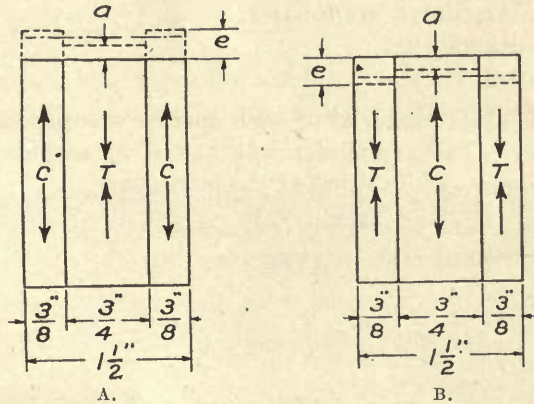
FIG. 4.—Combining high density and low density material in laminated construction.
