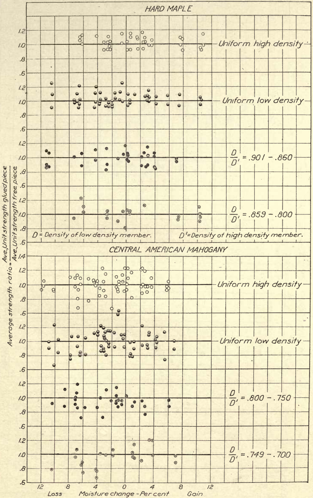
PLATE 17.—Results of tests showing relation between tensile strength across grain of laminated specimens (glued of uniform density and of non-uniform density stock) and tensile strength across grain of free specimens after both have been subjected to various atmospheric conditions.
