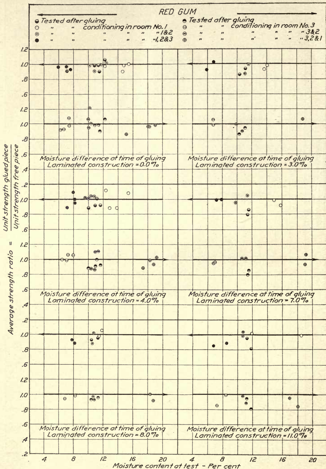
PLATE 14.—Results of tests showing relation between tensile strength across grain of laminated specimens (glued at uniform and at nonuniform moisture conditions) and tensile strength across grain of free specimens after both have been subjected to various atmospheric conditions.
