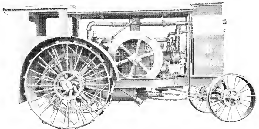
Mogul 30-60 H. P. Two Cylinder Oil Tractor
