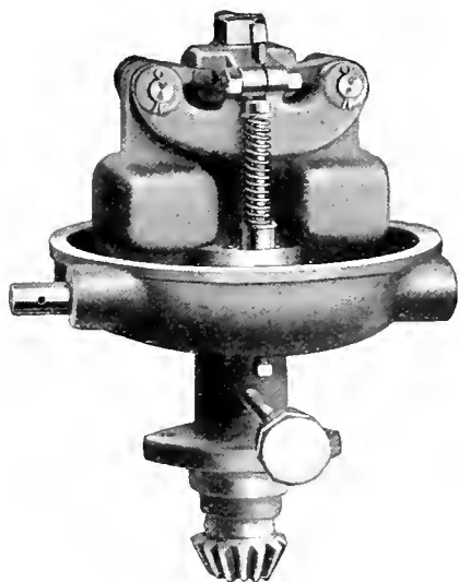
Governor with cap removed
