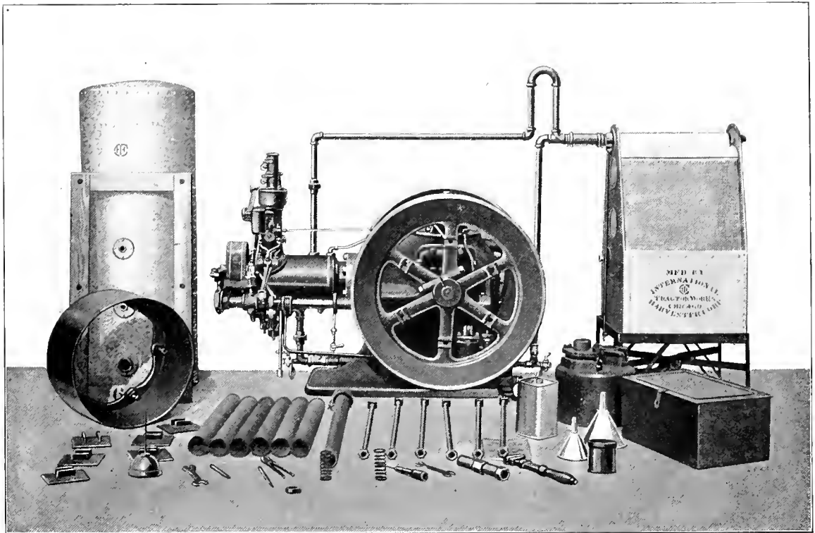
Mogul 4-H. P. Stationary Tank-Cooled Engine with complete equipment except fuel piping which is furnished as follows: 18 feet \frac{1}{4} -inch galvanized fuel pipe and 18 feet of \frac{3}{8} -inch galvanized overflow pipe
