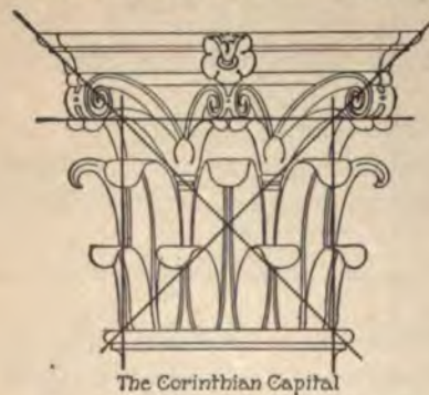
The Corinthian Capital FIG. 88
