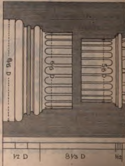
ELEVATION OF CAPITAL AND BASE
