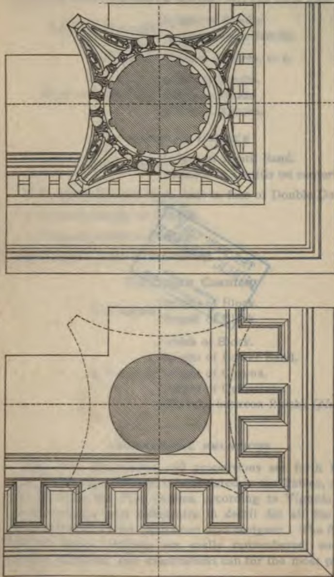
PLAN OF ENTABLATURES LOOKING UP
