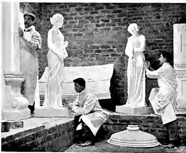
FIG. 5.—DRYING CHAMBER: CLEANING CASTS
