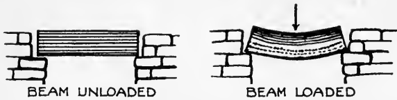
FIG. 29.—To show lines of compression (dark) and lines of tension (dotted) in a loaded rectangular beam. The clear space between the strut-lines and the tie lines indicates the neutral zone.
