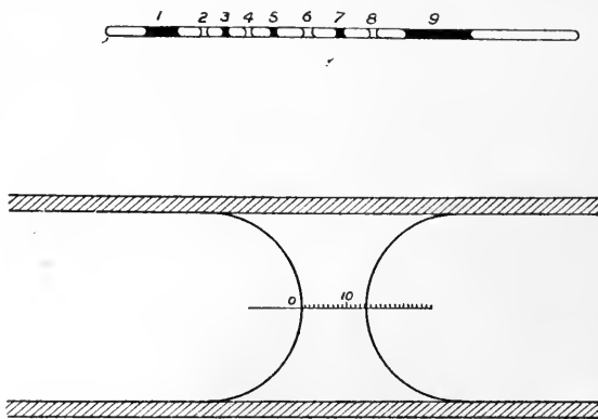
FIG. 75.—Barger's Method for determining Molecular Concentration.
