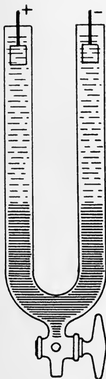
FIG. 9.—Apparatus for demonstrating cataphoresis. The deeply shaded lower portion of the U-tube is filled with a colloidal sol, the upper part with ordinary distilled water. On the passage of an electric current the colloid rises towards the electrode of opposite sign to the sol. (Hatschek.)
