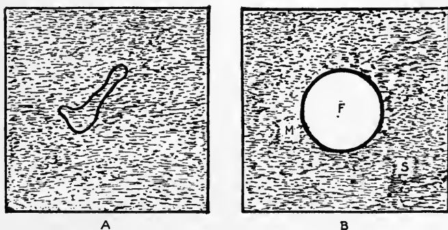
FIG. 24.—Frame of wire enclosing a Soap Film.
