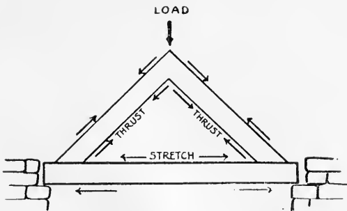
FIG. 30.—A simple triangular roof truss.
