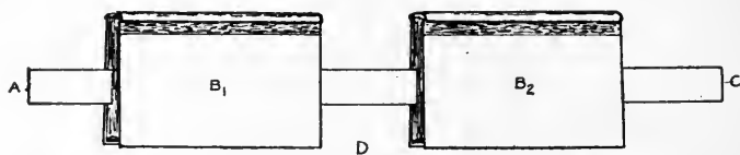
FIG. 13.—Model of polarimeter. A =source of light, B 1 =polariser, D =point at which twisting force is applied, B 2 analyser, the amount of twisting at D can be estimated from the angle through which B 2 has to be rotated to allow of the passage of the metal strip AC , C =eyepiece.
