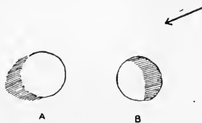
FIG. 54.—Shadows.
