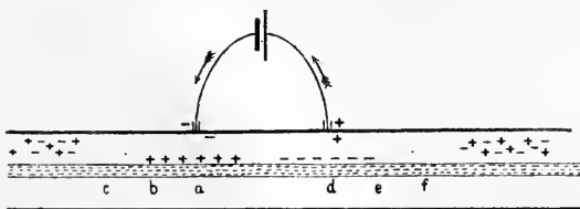
FIG. 38.—Diagram to show polarisation at the surface between conducting core and electrolyte sheath.
