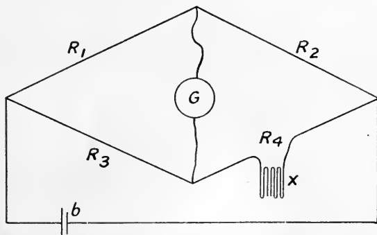
FIG. 78.—Diagram of Conductivity Apparatus.
