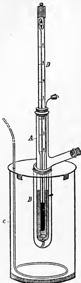
FIG. 74.—Freezing Point Apparatus.
