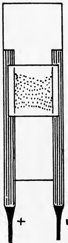
FIG. 10.—Apparatus for ultramicroscopic observation of the movements of colloids in an electric field (see Part II.). (Hatschek.)
