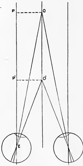
FIG. 52.—Convergence.
