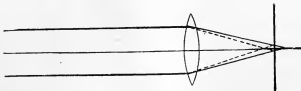
FIG. 48.—Chromatic Aberration.
