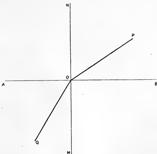
FIG. 46.—Refraction of incident ray PO at interface AB .
